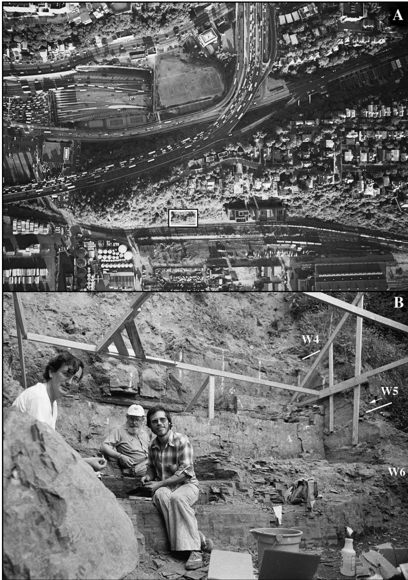
Fig. 4. Weehawken Quarry in Nursery Member of Locketong Formation. A , Aerial photograph of Kings Bluff area, Weehawken, N.J. showing the location of the Weehawken quarry (box), opened for Locketong vertebrates; illumination is from the bottom (east) during morning rush hour (photo courtesy William K. Sacco, 1978). B , The Weehawken Quarry in 1979 showing three cycles of the Nursery Member, including cycle W5 that produced abundant disarticulated Hypuronector (arrow) (photo courtesy of Amy R. McCune, 1979); people are, from left to right, Keith Stewart Thomson, Donald Baird, and Paul E. Olsen.
