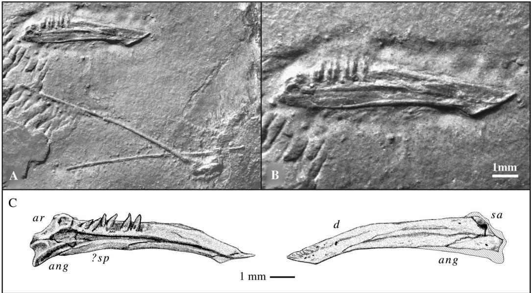
Fig. 8. Mandibles of Hypuronector : A , AMNH 2080, left mandible, medial view and associated caudal vertebrae from Granton Quarry; B , close up of mandible in A.; C , YPM 56388, lateral and medial views of negatively prepared specimen. Abbreviations are: d , dentary; ang , angular; ar , articular; sa , surangular; ?sp , ? splenial. Photograph by P. Olsen.
