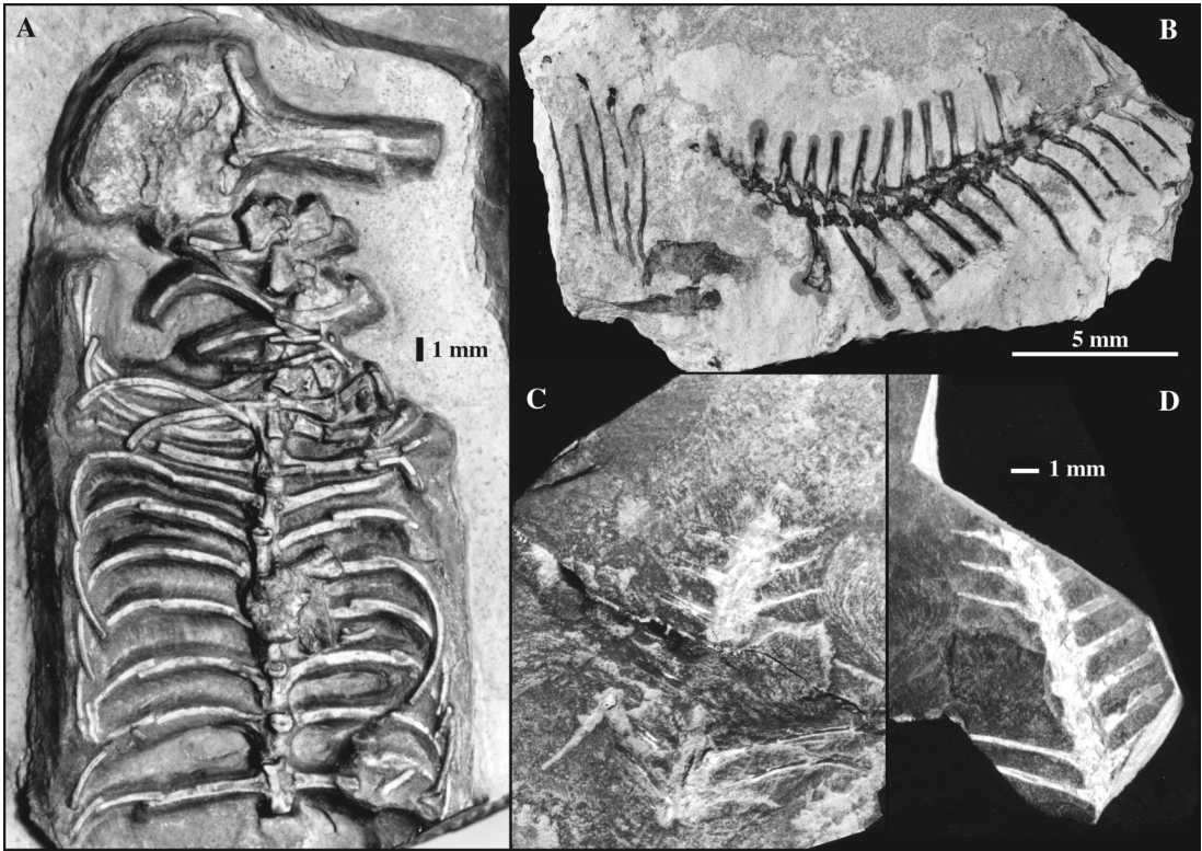
Fig. 7. Additional Granton Quarry specimens of Hypuronector . A , AMNH 1721, ventral view of trunk and left lateral view of crushed pectoral girdle. B , AMNH 7205, partial trunk, pelvic girdle, and proximal caudal vertebrae. C and D , AMNH 1998, unprepared part and counterpart of midcaudal vertebrae. Photographs by Chester Tarka, except for C and D by Julius Weber (courtesy of G. Case).
