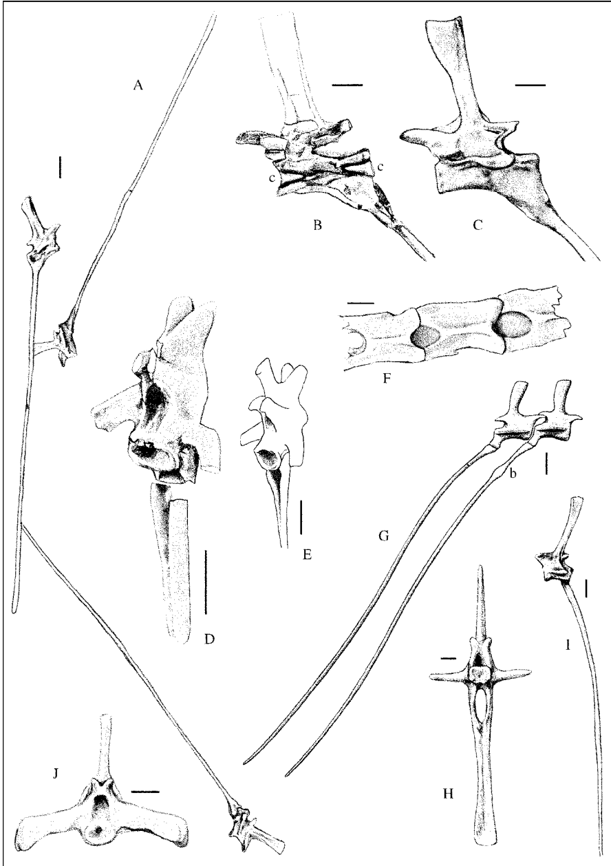
Fig. 9. Examples of vertebrae of Hypuronector (scale bar 1 mm): A , three associated caudal vertebrae with chevrons (YPM 56390); B , early stages of negative preparation of caudal vertebra and partial chevron (YPM 56389) showing matrix filling notochordal cones (c), shown reversed; C , same vertebra as B, fully prepared; D , negatively prepared, obliquely preserved caudal vertebra and partial chevron (YPM 56391); E , reconstruction of specimen in D; F , three cervical vertebrae in dorsal view (AMNH 7755); G , two successive caudal vertebrae and chevrons from the holotype (AMNH 7759); H , proximal caudal vertebra and chevron in anterior view (YPM 8641); I , isolated caudal vertebra and chevron (YPM 56387); J , isolated sacral vertebra in anterior view (YPM 56392).
