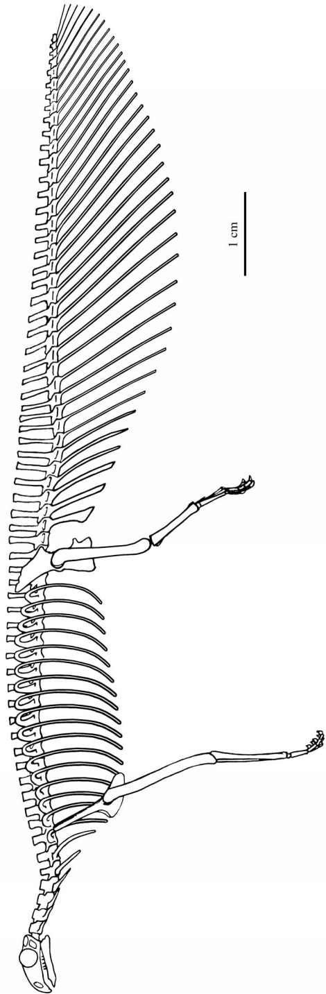
Fig. 15. Reconstruction of Hypuronector . The cranium and number of cervical vertebrae are conjectural.
