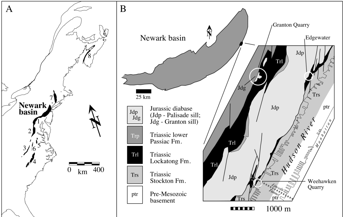
Fig. 1. Location of Hypuronector limnaios within the Newark Supergroup (A) and within the Newark basin of the Newark Supergroup (B). A , Map of the Newark Supergroup showing the outcropping basins. Major basins other than the Newark basin are: 1, Gettysburg basin; 2, Culpeper basin; 3, Dan River basin; 4, Deep River basin; 5, Richmond basin and associated Taylorsville basin to north; 6, Farmville and associated basins to south; 7, Hartford basin; 8, Fundy basin. Adapted from Olsen et al. (1996). B , Detailed map of Weehawken to Edgewater, New Jersey, area showing bedrock geology at major Hypuronector localities; based on Olsen (1980), Parker (1993), and Drake et al. (1996).
