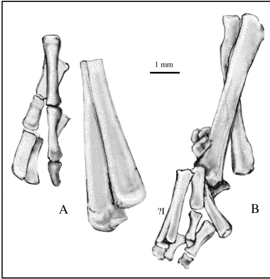
Fig. 13. Distal parts of the hind limb of Hypuronector . A , left hind limb; B , right hind limb. ?I, is possible proximal phalanx of digit I.
