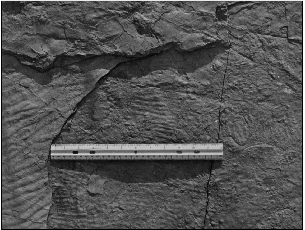
Plate V. Upper surface of unit 23b (above).
