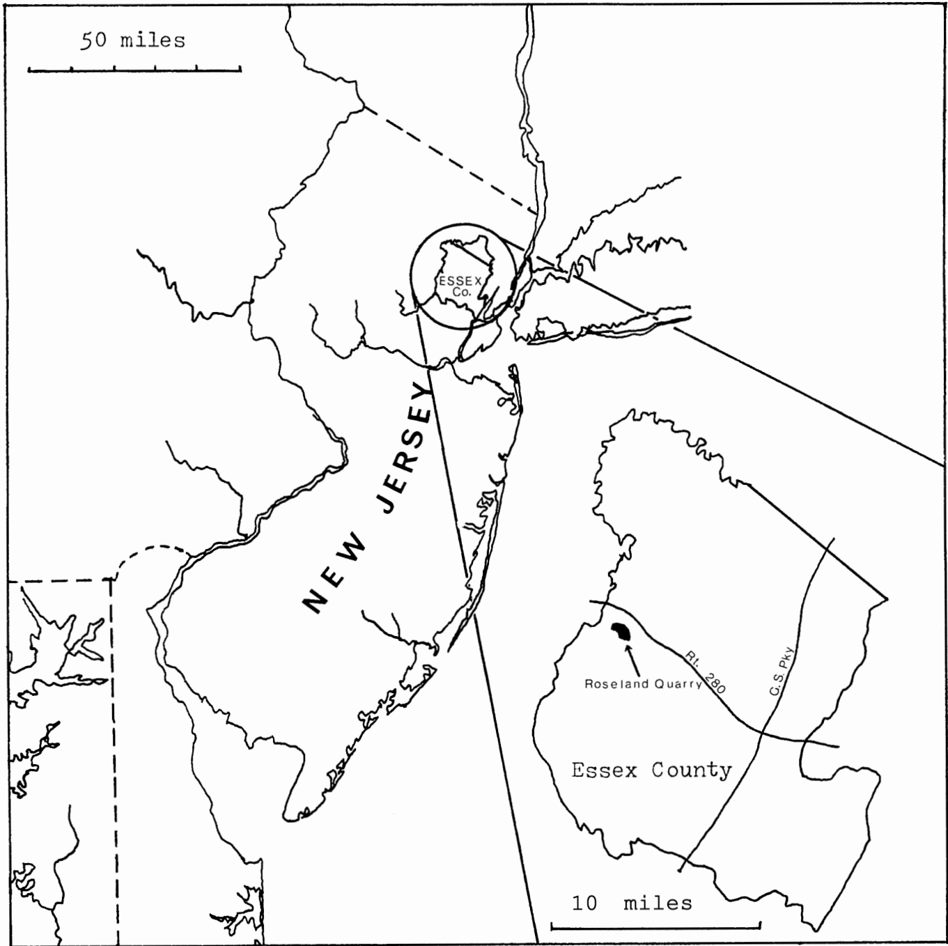
Figure 1. Geographic position of the Roseland Quarry.
