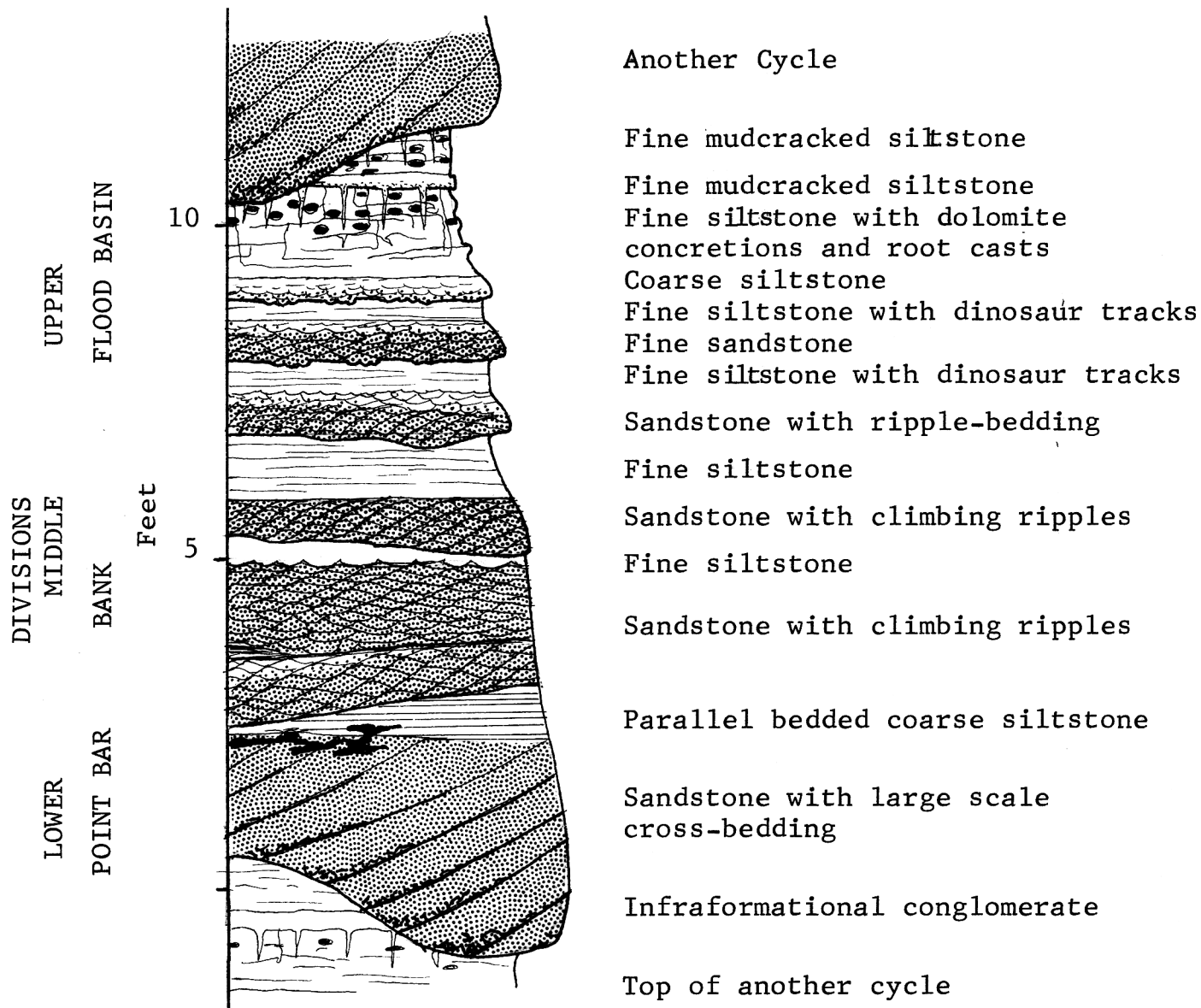
Figure 12. The modal fining-upwards cycle for the Towaco Formation.
