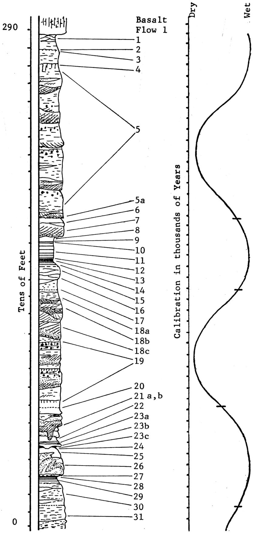
Figure 8. Key diagram for Roseland Quarry Section.
