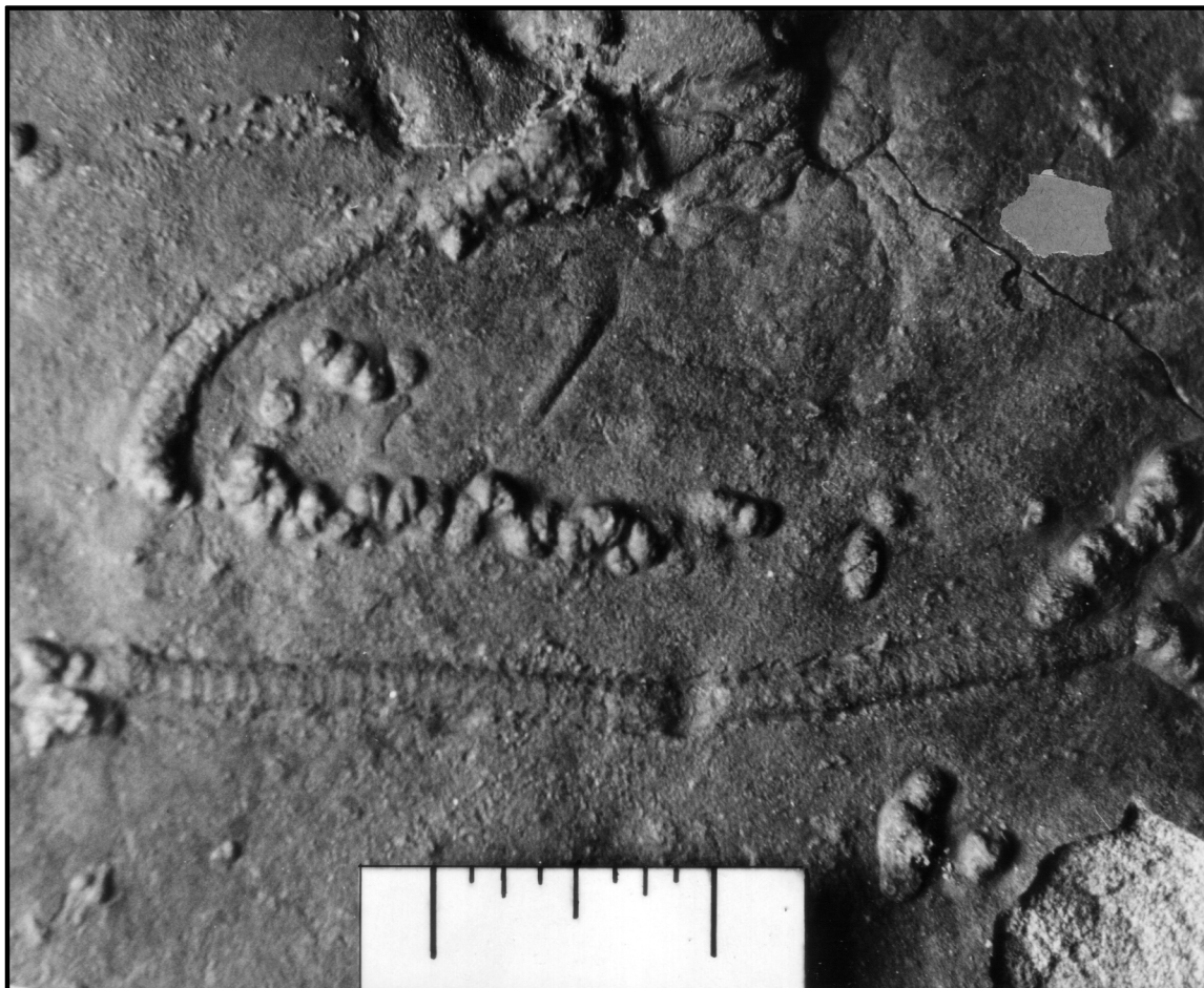
Plate XII. Worm burrows in lower surface of crevasse splay of unit 5. (above)
