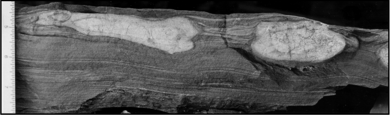
Plate IX. Dolomitic concretions in laminated red siltstone. Unit 19, second fining-upwards cycle (above). Scale in inches.
