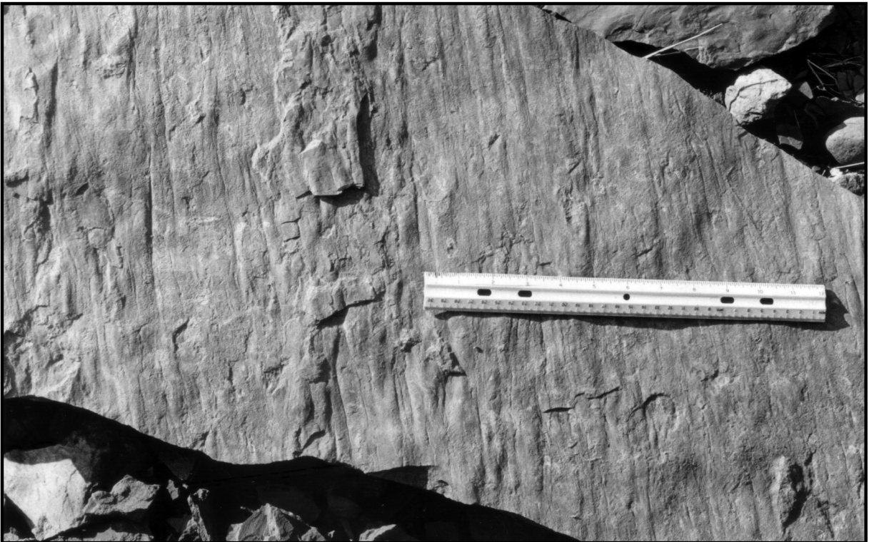
Plate VIII. Longitudinal grooves in base of channel of unit 19.
