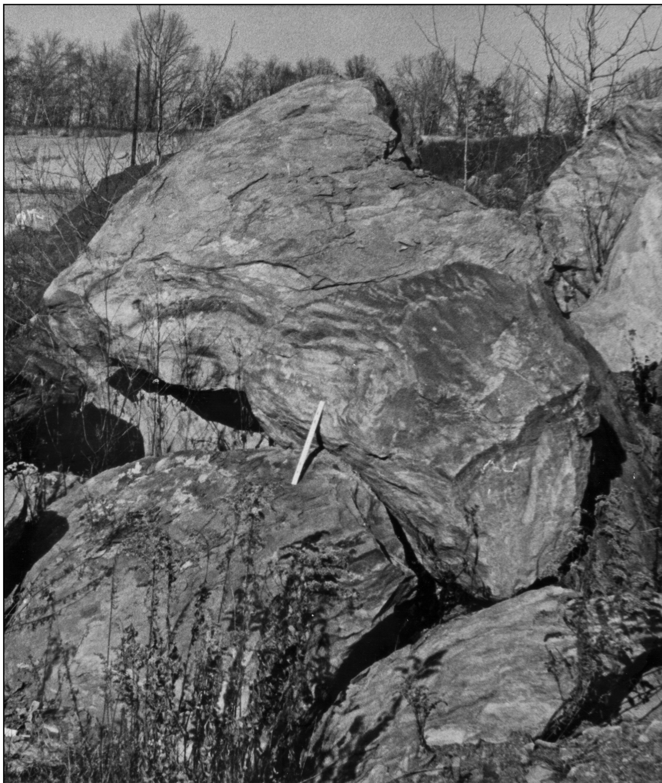
Plate III. Hook structures from unit 26. Ruler = 1 ft. photo by P. Olsen
