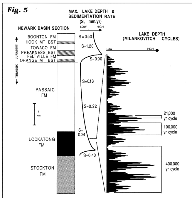
Fig. 5: Stratigraphic pattern seen in the Newark Basin. Maximum lake depth is simply the enveloping surface of the Milankovitch-period lake-level fluctuations, which represents the maximum depth lakes attained during the wettest of climate cycles. The thicknesses of the 21,000-year cycles were used to calculate the sedimentation rates in this figure.
