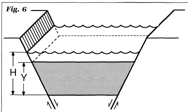
Fig. 6: Full-graben model used to generate curves in Fig. 7. A full-graben is a symmetrical basin bounded on both sides by normal faults (shown by the half-arrows). As the graben grows larger and larger through time, the thickness of sediment deposited per unit time must decrease. Y is the cumulative sediment thickness, and H is equal to maximum lake depth plus Y .
