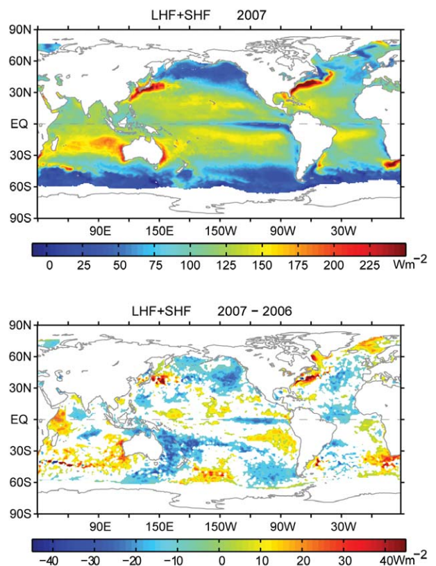
Fig. 3.7. (top) Annual mean latent plus sensible heat fluxes in 2007 (in W m^{-2} ). (bottom) Differences between the 2007 and 2006 annual mean latent plus sensible heat fluxes (in W m^{-2} ). The sign is defined as upward (downward) positive (negative). The differences significant at the 90% confidence level are plotted.
