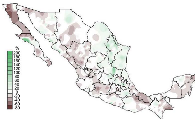
FIG. 6.16a. Mexican seasonal rainfall anomalies (May–Oct) in 2007.
