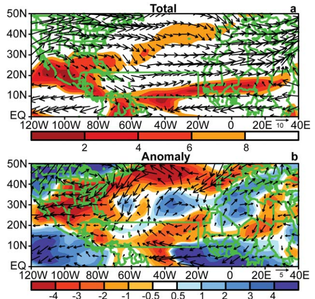
FIG. 4.12. Aug–Oct 2007: 200–850-hPa vertical wind shear magnitude ( m s^{-1} ) and vectors (a) total and (b) anomalies. In (a), shading indicates vertical wind shear below 8 m s^{-1} . In (b), red (blue) shading indicates below- (above) average magnitude of the vertical shear. Green box denotes the MDR. Vector scale is shown at bottom right of each panel. Anomalies are departures from the 1971–2000 period monthly means.
