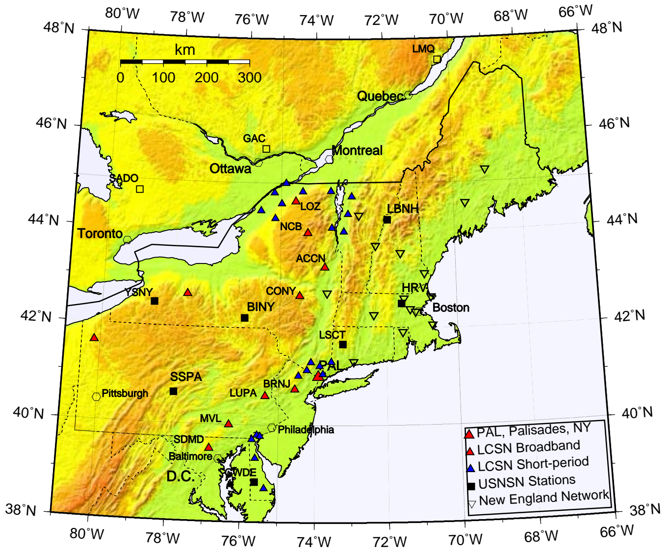
Figure 1. Seismographic stations of the Lamont-Doherty Cooperative Seismographic Network (LCSN) and other stations in the Northeastern U.S. LCSN broadband stations (red triangle), LCSN short-period stations (blue triangle), broadband stations of the USNSN (black square), New England Seismic Network (inverted triangle) and Canadian National Seismic Network (CNSN; open square) are plotted for reference.
