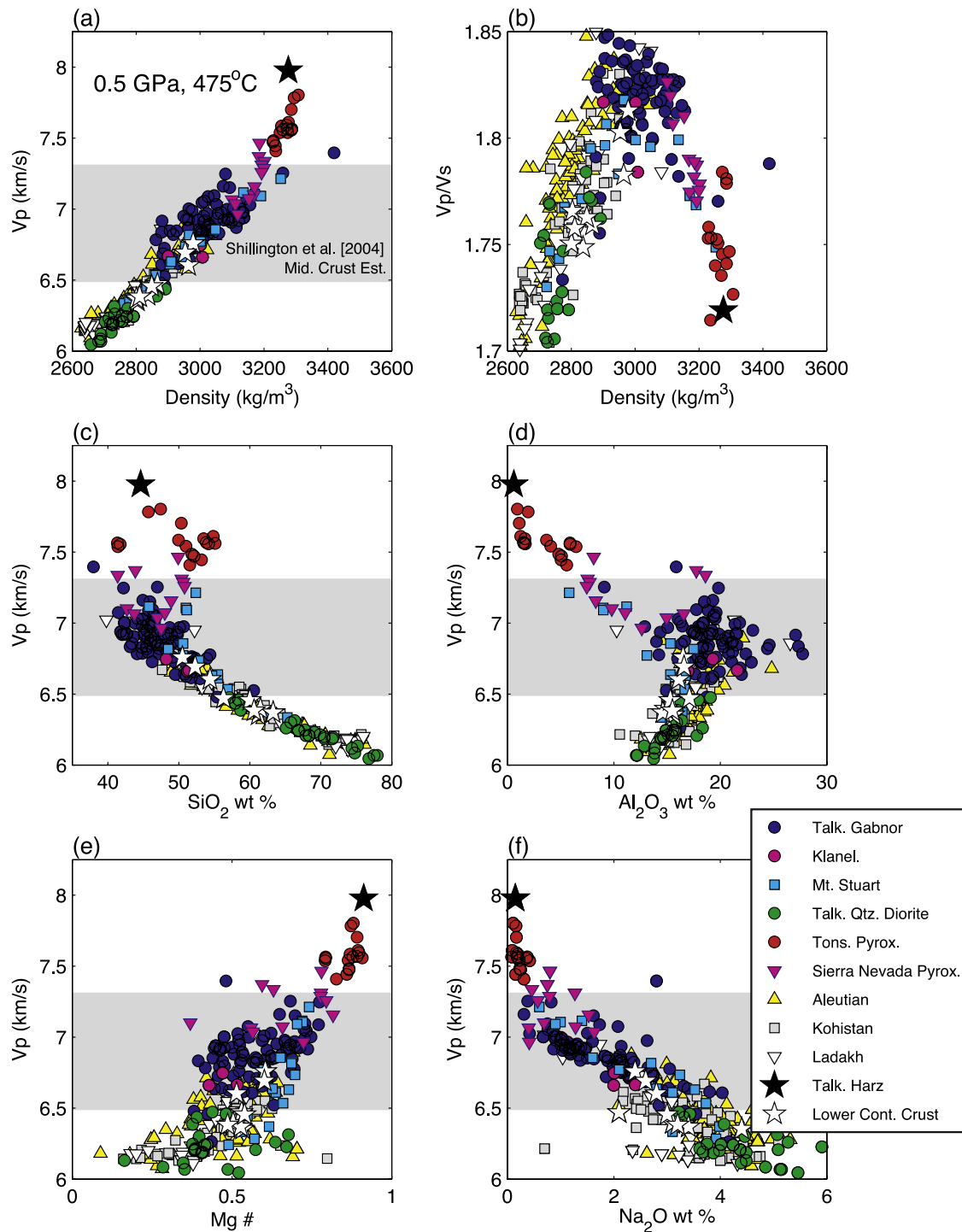
Figure 11. Comparison of (a) calculated Vp and density and (b) calculated Vp/Vs and density for a range of arc compositions at midcrustal conditions (475°C and 0.5 GPa). (c–f) Calculated Vp versus SiO 2 , Al 2 O 3 , Mg #, and Na 2 O, respectively. Grey band indicates midcrustal P wave velocities (6.5–7.3 km/s) for the central Aleutians island arc from Shillington et al. [2004]. See Figure 10 for full description of symbols and calculations.
