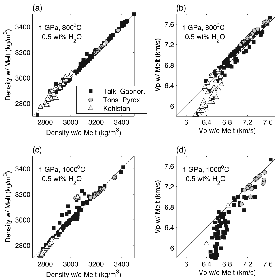
Figure 13. Effect of melting on density and Vp for a range of gabbro and pyroxenite compositions from the Talkeetna and Kohistan arc sections. Calculations are performed at (a,b) 800°C and (c,d) 1000°C and 1 GPa and assume 0.5 wt % H 2 O. Effect of melt on Vp is calculated after Mainprice [1997], assuming spherical melt inclusions and a melt bulk modulus of 15 GPa. For seismic velocities typical of arc lower crust (6.9–7.3 km/s) melting has a small influence on both density and Vp.
