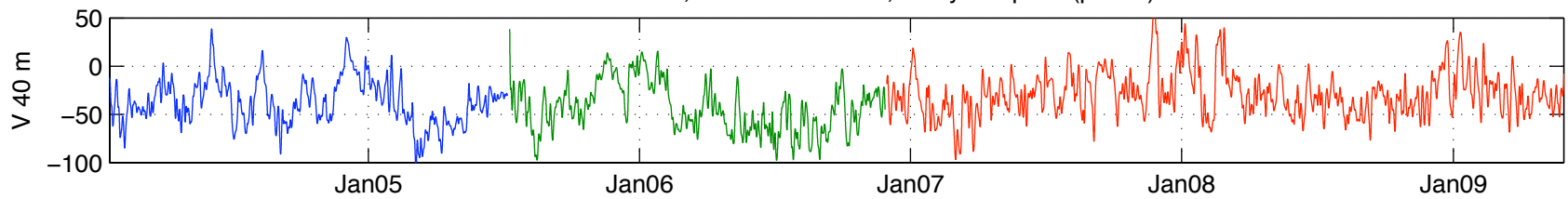
Mak West 1&2, ITF06-09 V cm/s, 3 day low pass (prelim)
