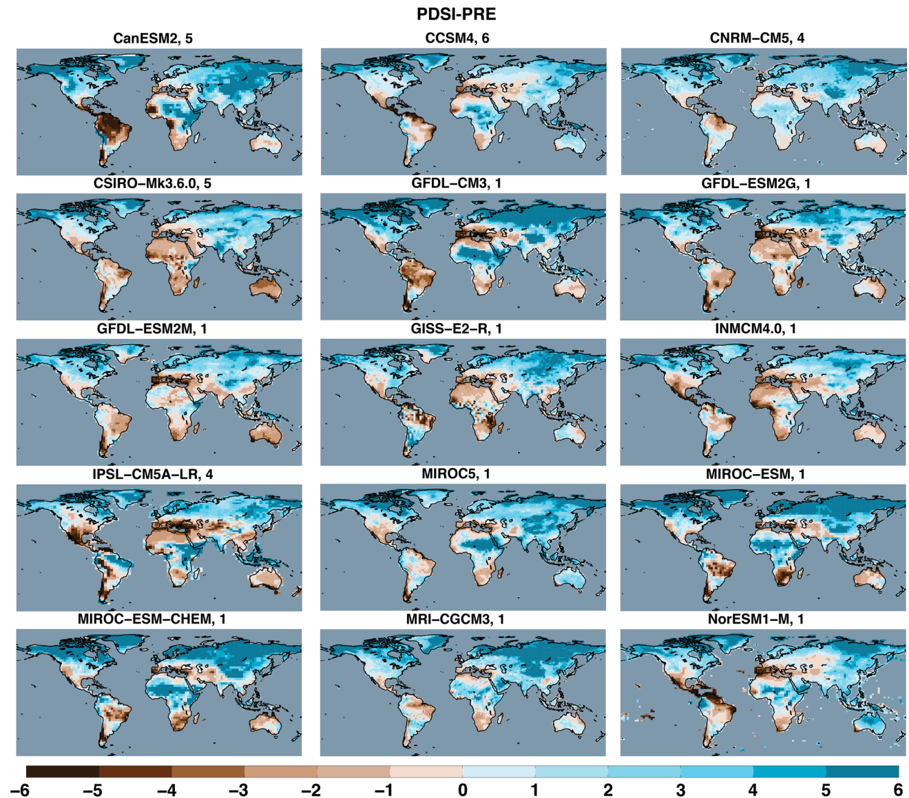
Fig. 7 Annual averaged PDSI-PRE (precipitation effects only) for each model simulation under the RCP8.5 scenario. The number of ensemble members is listed in each panel title; for models with multiple ensemble members, the maps represent the ensemble average
