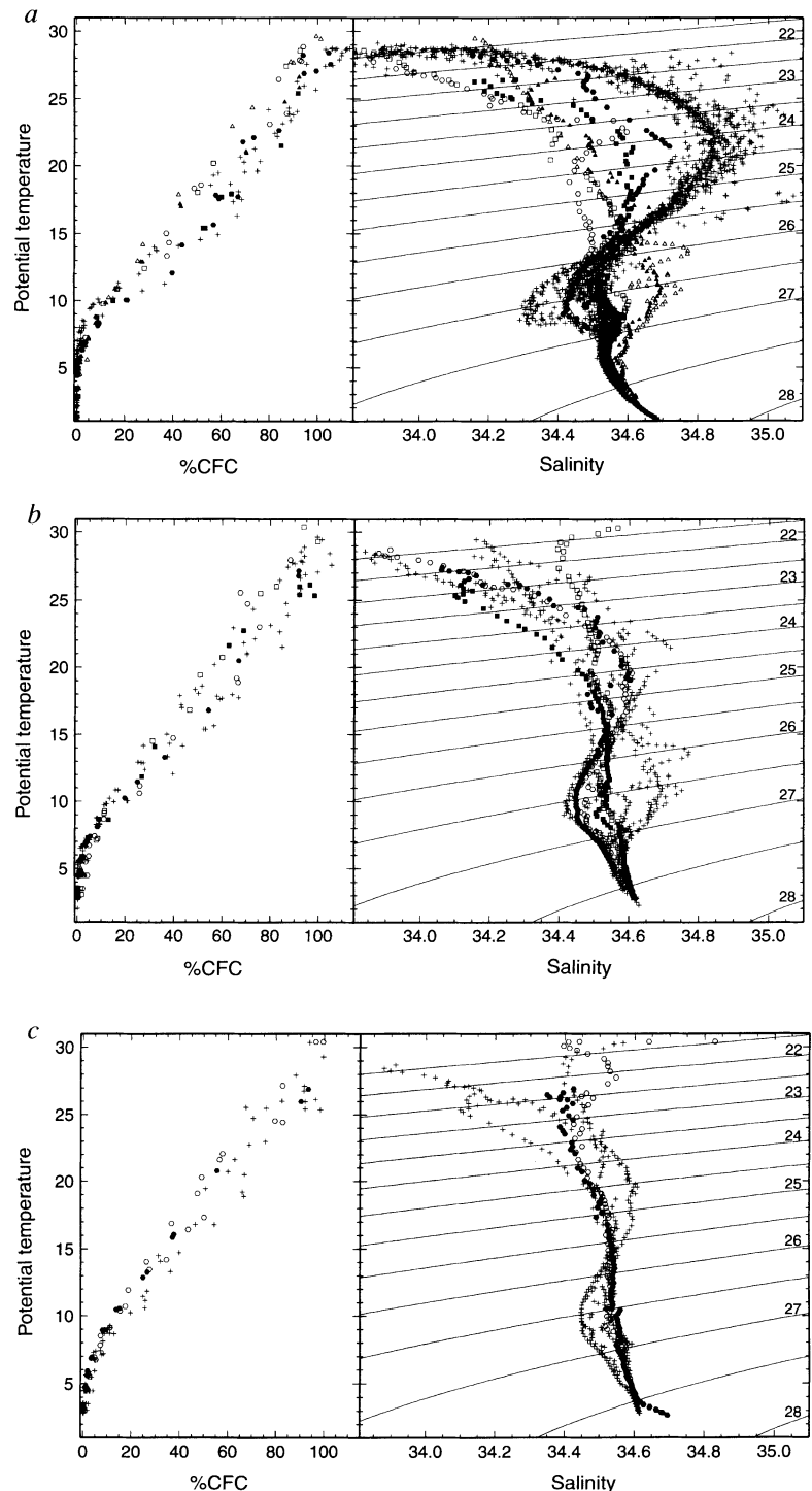
FIG. 3 Scatter plots of potential temperature/salinity ( T/S ) and potential-temperature/percentage saturation CFC-11 ( T/\%CFC ) relationship for selected stations within the Indonesian Seas. The curved lines within the T/S plot marked 22–28 are lines of equal density (isopycnals) in \sigma_\theta nomenclature. Due to the sparser resolution for CFCs, multiple and nearby stations are used to fill out the \%CFC profile. Solid symbols represent the southeast Monsoon (SEM); open symbols represent the northwest Monsoon (NWM). a, The northern Indonesian seas. Circles show Makassar Strait stations, the T/S data are derived from stations 21 and 186; the \%CFC data are derived from the stations 17, 18, 21, 186, 189 and 190 for the NWM. Boxes show the Maluku Sea, the T/S data are derived from stations 29 and 177; the \%CFC data are derived from the stations 30 and 176. Triangles show the Seram Sea, the T/S data are derived from stations 38 and 168; the \%CFC data are derived from the stations 38, 39, 167 and 169. R/V Moana Wave stations 3–36 (stations from May 1989 spanning the Mindanao Current west of 140° E between 8° and 9° N; ref 23) are shown as a +, as reference for the Arlindo T/S and T/\%CFC scatter. The Moana Wave stations west of 127.67° E (within 115 km of the continental shelf) are responsible for the low-salinity feature in the 8–13 °C temperature interval, making a rather abrupt transition from more saline water to the east. It is this water that can be traced into the Makassar Strait. b, The southern Indonesian seas. Circles show the Flores stations, the T/S data are derived from stations 93 and 116; the \%CFC data are derived from the stations 96, 97, 113 and 114. Boxes show the Banda Sea, the T/S data are derived from stations 71 and 138; the \%CFC data are derived from stations 70, 71, 138 and 139. The northern data (from Fig. 3a) are shown as a + for reference. c, Timor Sea. Circles shows the T/S and T/\%CFC relation for the Timor Sea, the T/S data are derived from stations 75 and 130; the \%CFC data are derived from the stations 74, 75, 128, 129, 130. The Flores and Banda sea (Fig. 3b) are shown as a + for reference.
