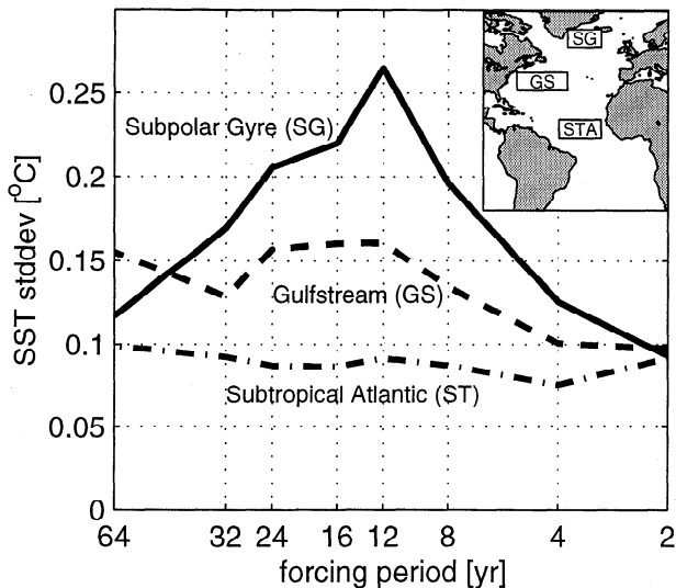
Figure 2. Model winter SST standard deviation as a function of forcing period for the Gulf Stream, Subtropical Atlantic, and subpolar gyre regions (see map for locations). The selected regions are: Gulf Stream ( 31^{\circ} - 41^{\circ} N, 70^{\circ} - 40^{\circ} W), tropical/subtropical Atlantic ( 5^{\circ} - 15^{\circ} N, 44^{\circ} - 20^{\circ} W) and the subpolar gyre ( 55^{\circ} - 65^{\circ} N, 40^{\circ} - 30^{\circ} W).
