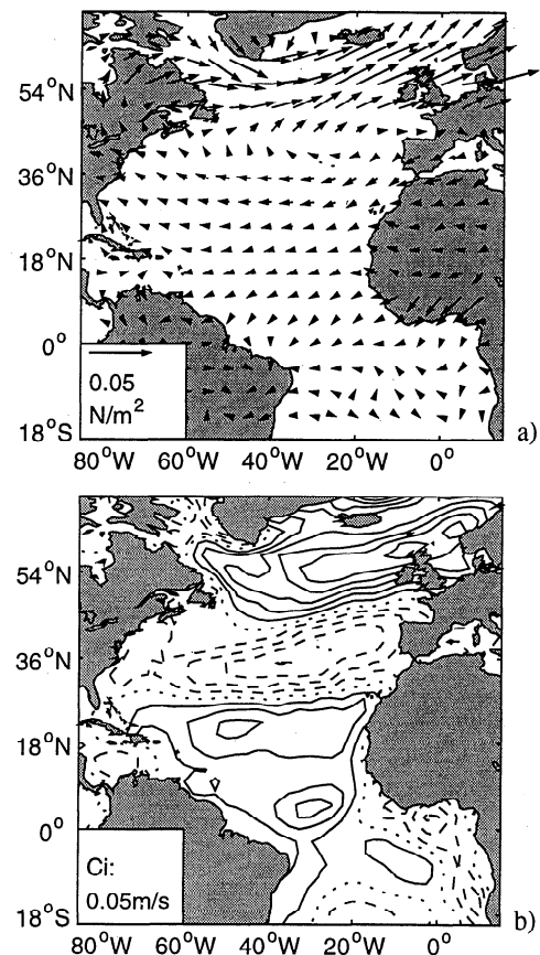
Figure 1. a) Wind stress anomalies per NAOI unit obtained by regressing the November-April NCEP NCAR Reanalysis (1958-1998) against the Hurrell NAO index (see text for details); b) same as a) but for wind speed.
