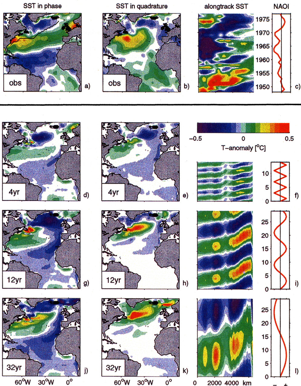
Plate 1. a) Observed in-phase SST response during the NAO+ phase based on the COADS SST data set (see text for details); b) In-quadrature response with a 90° phase lag after the NAO+ phase (see text for details); c) SST anomalies as a function of distance and time along a path from Florida to Scotland (depicted in a) by a solid black line). The next three rows display the 4, 12, and 32 year ocean model SST response. The first column (d,g,j) shows the annual mean SST response in phase with the NAO index. The middle column (e,h,k) shows the in-quadrature response. The right column (f,i,l) displays the model SST anomalies as a function of distance and time as in c).
