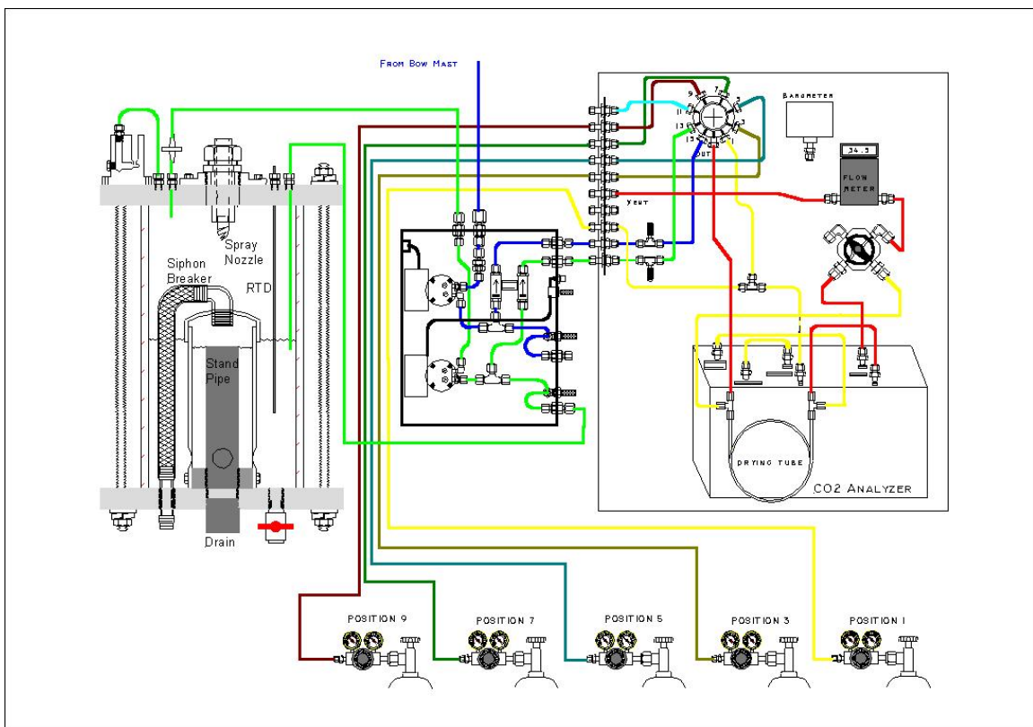
Figure 1 - The underway pCO 2 system used for the measurements of pCO 2 in surface waters installed in early December 2003.
