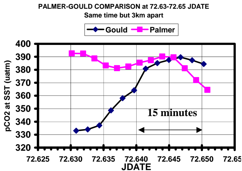
Figure 3 – Surface water pCO_2 and SST data obtained aboard the Gould and Palmer at the same time. The ships were 3 kilometers apart during the 15 minute period indicated by the arrow.
