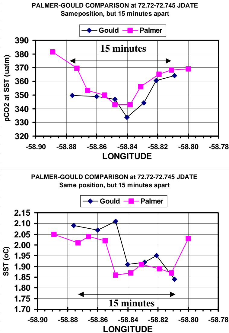
Figure 5 – Surface water pCO_2 and SST data obtained aboard the Gould and Palmer as the ships sailed along the same track (Period D in Fig. 1). The Palmer was trailing the Gould by about 15 minutes. The arrow shows the period of 15 minutes, during which the data are compared.
