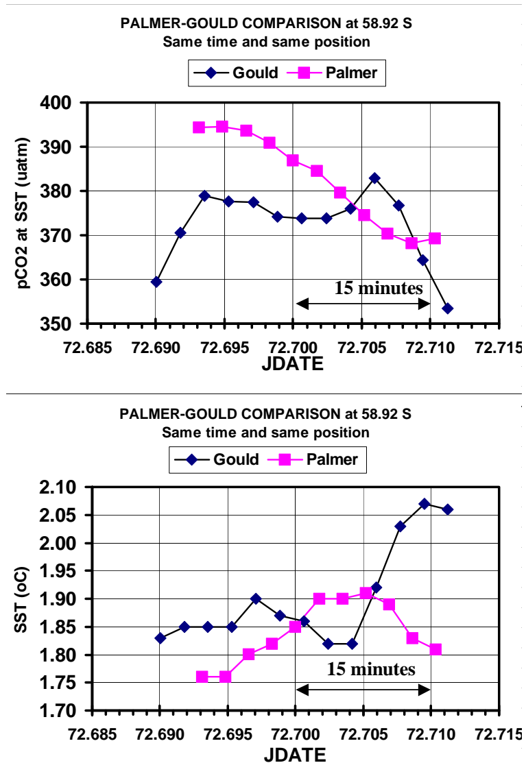
Figure 2 – Surface water pCO 2 and SST data obtained aboard the Gould and Palmer at the same time when the ships were less than 300 meters apart.
