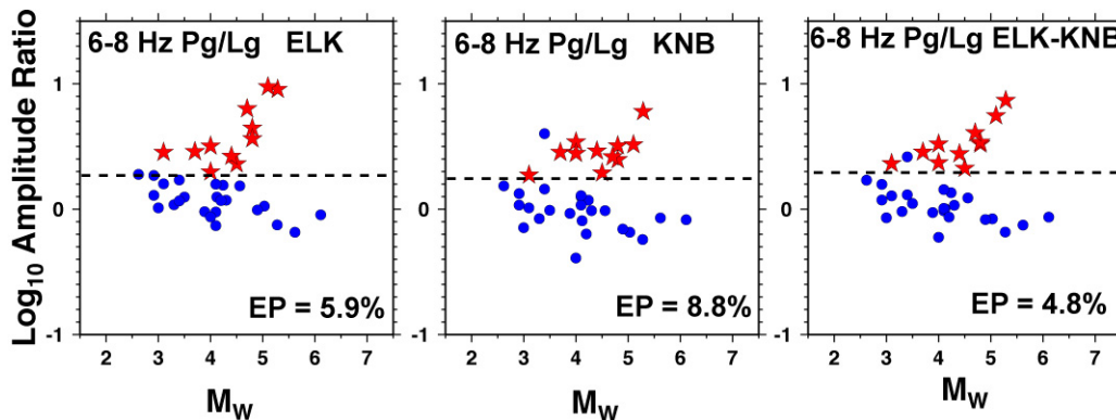
Figure 6. Comparison of 6–8 Hz Pg/Lg discrimination performance at stations ELK and KNB for the same events. ELK has better performance than KNB. An earthquake outlier at KNB is not an outlier at ELK indicating that averaging should help reduce variance. A hypothetical decision line has been drawn just below the lowest explosion value in each case. Note that the average of the two stations performs better than either alone as measured by equiprobable value.
