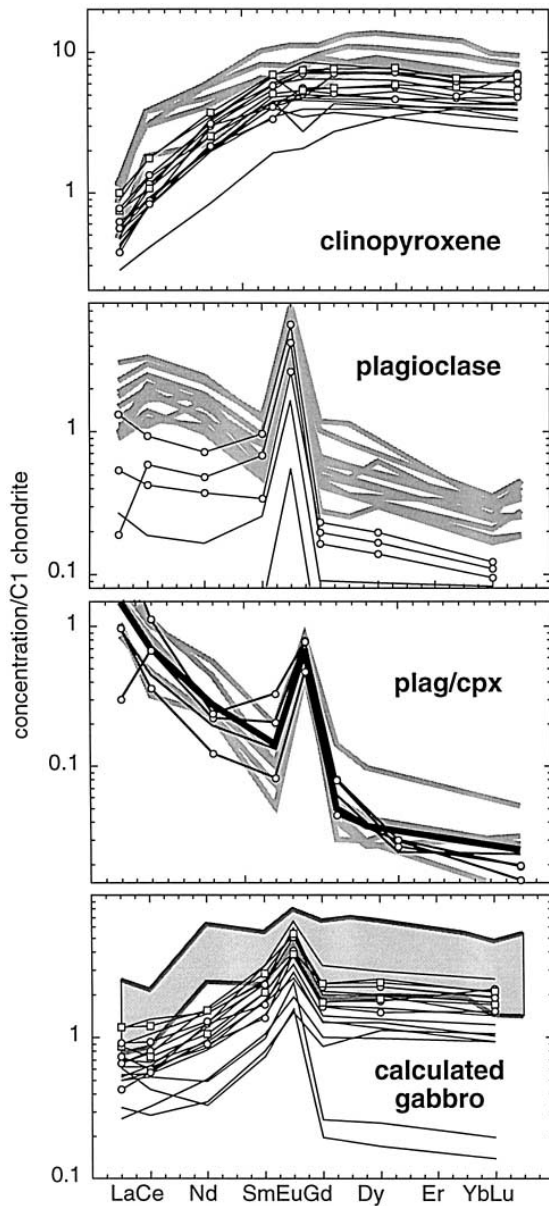
Fig. 4. Average REE concentration in minerals from layered gabbros from the Ibra and Maqsd areas, normalized to concentration in C1 chondrites [76]. Solid lines are for samples from the Maqsd area analyzed by ion microprobe at Woods Hole (see EPSL Online Background dataset , table 1, also available from the authors). Lines with open symbols are for 6 lower crustal gabbros; lines without symbols are for 12 sills in the MTZ. Light gray lines are instrumental neutron activation analyses (INAA) of mineral separates from lower gabbros in the Ibra area [15]. Top: clinopyroxene compositions. Second panel: plagioclase compositions. Third panel: plagioclase/clinopyroxene concentration ratio. Heavy dark line is average incorporating both our data and [15] (see EPSL Online Background dataset , table 2). Bottom: calculated gabbro compositions for Maqsd area, using ion probe analyses of clinopyroxene, average plagioclase/clinopyroxene distribution coefficients, and estimated modal proportions of minerals in each sample ( EPSL Online Background dataset , table 1). The shaded field outlines the range of whole rock compositions of lower gabbros in the Ibra area measured by INAA [15]. Positive Eu anomalies in Oman lower gabbros are indicative of a cumulate origin.
