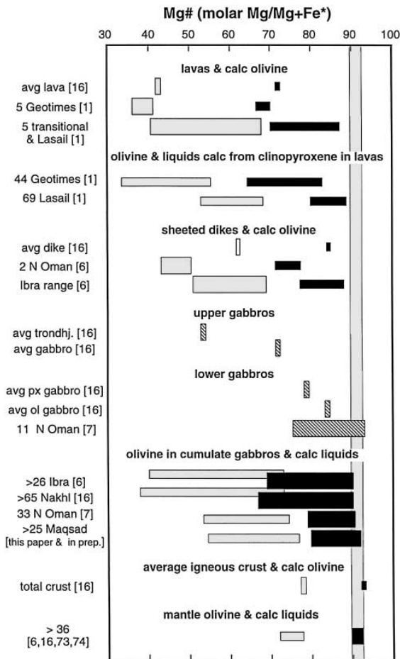
Fig. 2. Compiled data on percent Mg# (100 molar Mg/(Mg + Fe 2+ )) for whole rocks and minerals from the Oman ophiolite. Weight ratio of Fe 2+ /Fe 3+ in liquids assumed to be 0.9. “Liquids” (lavas, dikes and calculated liquids) are shown as light gray bars; plutonic rocks as dark gray bars; olivines as black bars. For each lava and dike, equilibrium olivine Mg# has been calculated using molar [Fe 2+ /Mg (olivine)]/[Fe 2+ /Mg (liquid)] = 0.3 [72]. Conversely, where mineral compositions were measured, liquid compositions have been calculated. For clinopyroxene, we used molar [Fe 2+ /Mg (clinopyroxene)]/[Fe 2+ /Mg (liquid)] = 0.25. Measured values are shown as wide bars, calculated values as narrow bars. Number and sources of data are given in legend on left. In legend, “Geotimes” and “Lasail” are the two oldest and most voluminous lava units, “Ibra”, “Nakhl” and “Maqсад” are massifs in the south half of the ophiolite, and “N. Oman” refers areas in the north half of the ophiolite. None of the lavas and dikes have Mg# as high as primitive, mantle-derived liquids. Instead, all must have evolved by crystal fractionation from a primitive parental liquid. Olivine in lower gabbros has Mg# appropriate for Fe/Mg equilibrium with the liquids that formed the lavas and dikes. Thus, lower gabbros may be interpreted as “cumulates”, from which the liquids that formed the upper crust were extracted. Data from [1,6,7,16,73,74].
