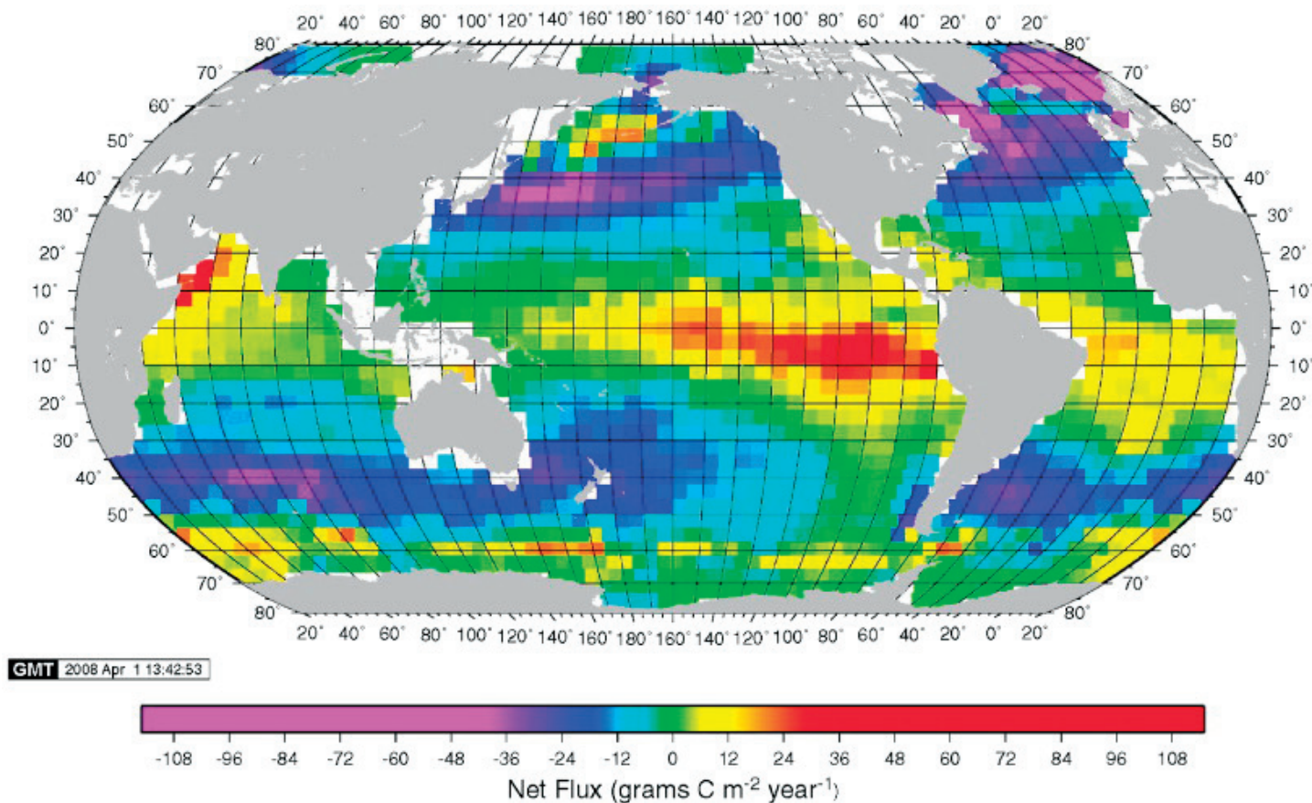
Figure 2. Climatological mean annual sea-air CO 2 flux (g-C m -2 yr -1 ) for the reference year 2000 (non-El Niño conditions) from Takahashi et al., 2009.
