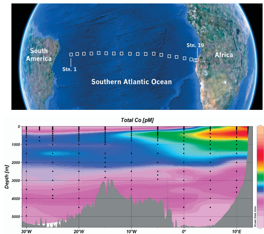
Figure 1. Top panel: Cruise track from the CoFeMUG South Atlantic cruise in November 2007 (Chief Scientist: Mak Saito). The main zonal section was sampled to full-depth for bioactive trace metals and nutrients.
