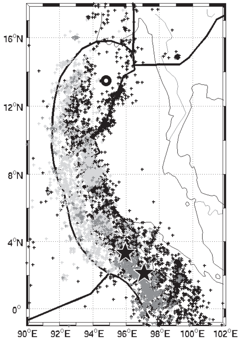
Seismicity from 1973/2/16 - 5/14/2005 (NEIC)
