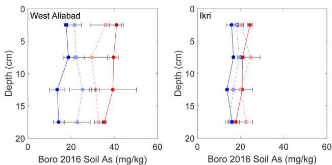
Figure 2. Depth profiles over the top 20 cm from two representative study sites. Arsenic profiles measured over the top 20 cm of soil for the low As control (dark blue), low-replaced-by-high (light blue), high-replaced-by-low (light red), and high As control (dark red) plots during the boro 2016 season for a. West Aliabad and b. Ikri. These figures represent the average across monthly samples taken four times from each plot during the growing season. Error bars represent standard deviation divided by the square root of the number of samples.
