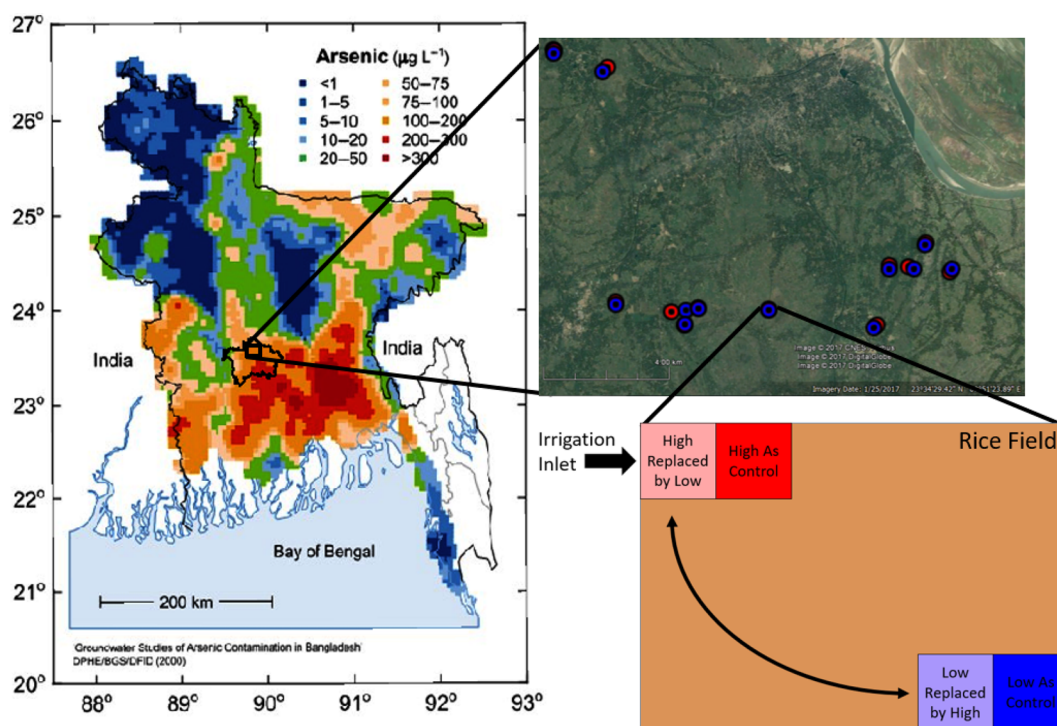
Figure 1. Soil exchange schematic and distribution of the 13 study sites within a 150 km 2 area in Faridpur, Bangladesh. The top 15 cm of soil was exchanged between a 5 × 5 m high-arsenic plot near the irrigation inlet and a 5 × 5 m low-arsenic plot far from the irrigation inlet. Adjacent 5 × 5 m control plots remained undisturbed and were managed identically to the soil replacement plots. Heat map of As in groundwater is reprinted from BGS; DPHE. Arsenic contamination of groundwater in Bangladesh Vol 1: Summary. In British Geological Survey Technical Report WC/00/19 ; Kinniburgh, D. G., Smedley, P. L., Eds.; British Geological Survey: Keyworth, 2001; Vol. 1. 36 Copyright 2001 BGS and DPHE. Map data is from Google, CNES/Airbus, and DigitalGlobe.
