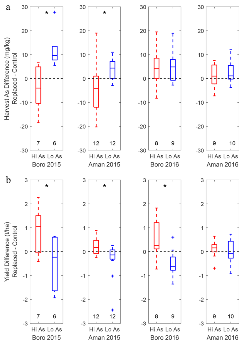
Figure 3. Soil As and yield differences between replacement and control plots. a. Differences in soil As between the replaced and adjacent control plots over the top 20 cm as measured by XRF on cores collected at harvest. b. Differences in rice yield between the replaced and adjacent control plots. Data are shown for all plots where yield was measured in each growing season, and the numbers below each box indicate the number of pairs of plots that box represents. The tops and bottoms of each box are the 25th and 75th percentiles. The line in the middle of the box shows the sample median. Outliers are values that are more than 1.5 times the interquartile range beyond the edge of the box. Asterisks denote a significant difference in medians at p = 0.05 according to an unequal variance t test.
