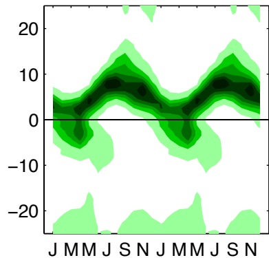
ERA40
