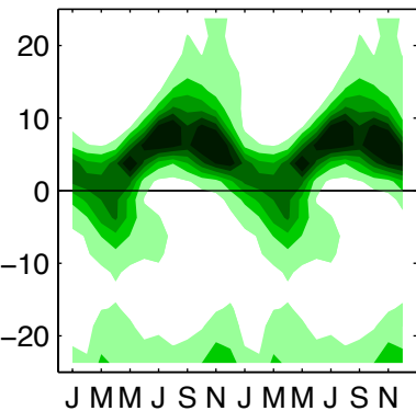
NCEP1
