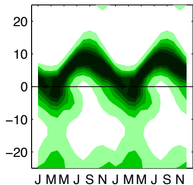
ECHAM4.5
