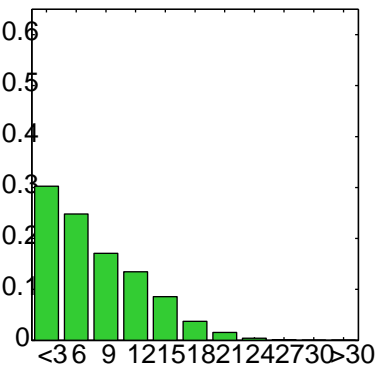
NCEP1
