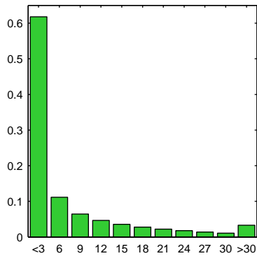
GPI
