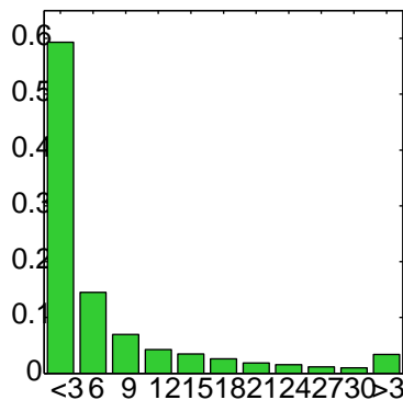
ECHAM4.5
