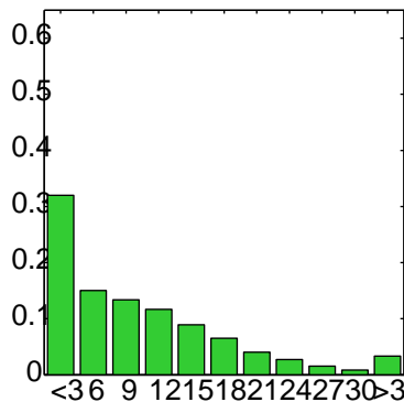
ERA40
