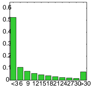
NCEP2
