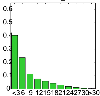
GFDL_AM2
