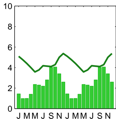
ERA40
