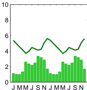
NCEP2
