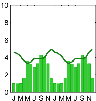
NCEP1
