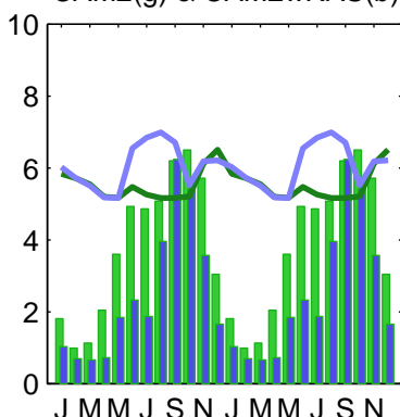
GFDL_AM2
