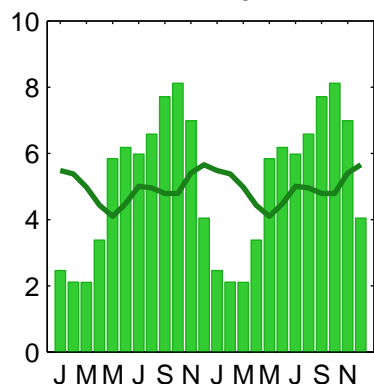
ECHAM4.5
