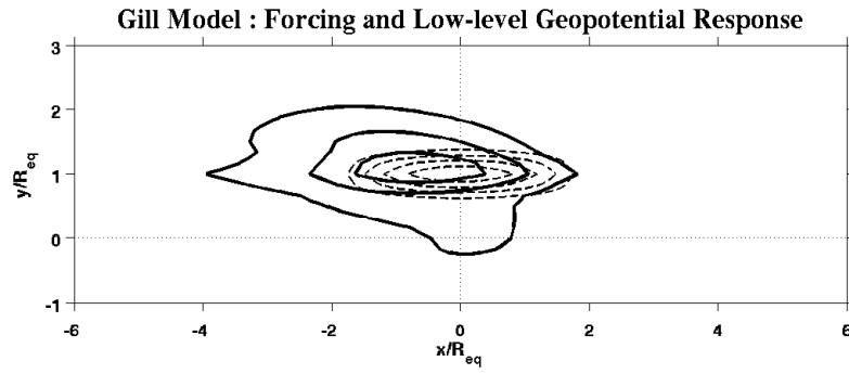
Figure 13. The low-level geopotential response (thick solid line) to a negative heating forcing (thin dashed line) in a Gill-like model (see text for details).
