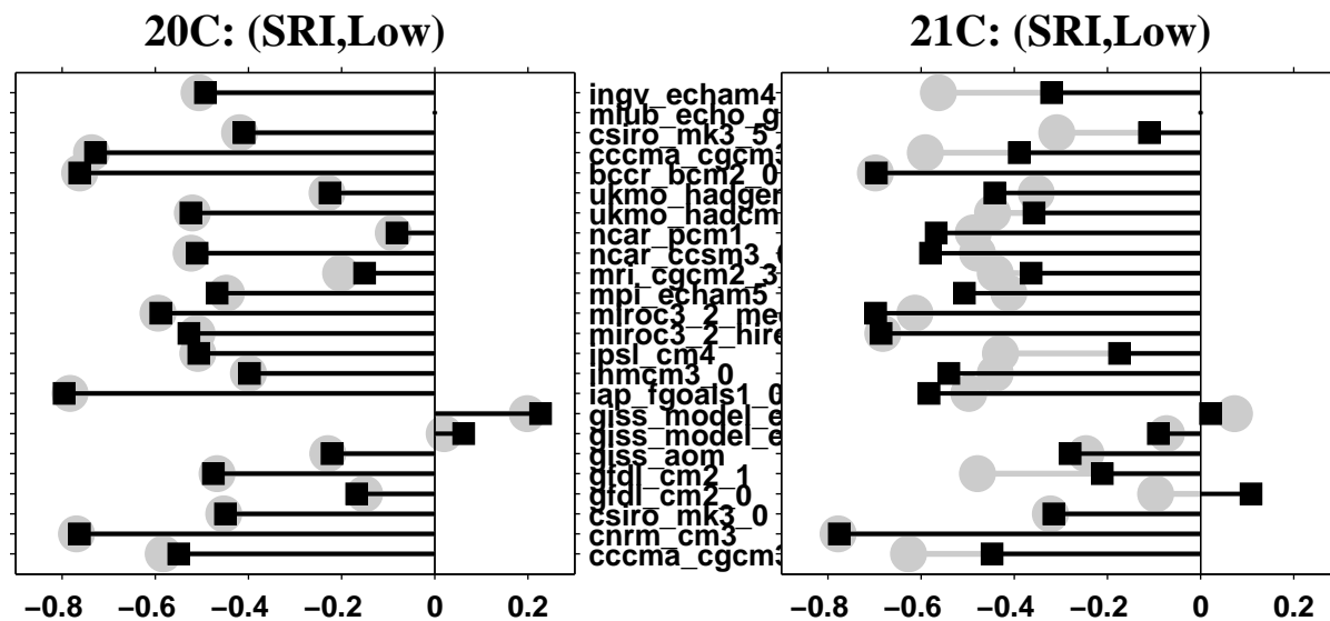
Figure 9. Correlation between the Sahel Rainfall Index (JAS rainfall averaged over the area between 10N-20N and 20W-40E) and the Sahara Low Index (the difference between Sahara average (20N-30N; 10W-30W) and tropical average (30S-30N) geopotential at 925hPa) in (left) 20C and (right) 21C. Circles indicate correlations between detrended time series, squares between unfiltered time series. Interannual correlations above \pm 0.16 are significant at the 95% level.
