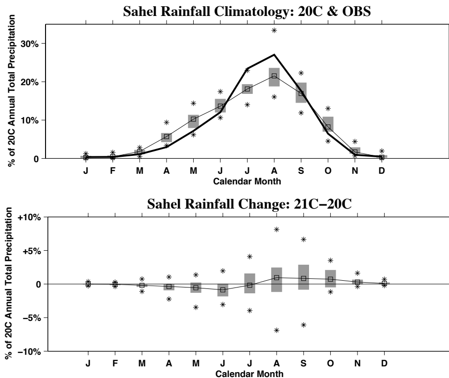
Figure 1. CMIP3 simulations of (top) 20C Sahel rainfall and (bottom) 21C-20C Sahel rainfall change (% of total annual rainfall) as a function of calendar month. The solid line and open squares show the mean anomaly, the grey vertical bars represent the 25th and 75th percentile, and the stars are the maximum and minimum values. The thick black line in the upper panel is observations (Hulme, 1992) for 1975-1998.
