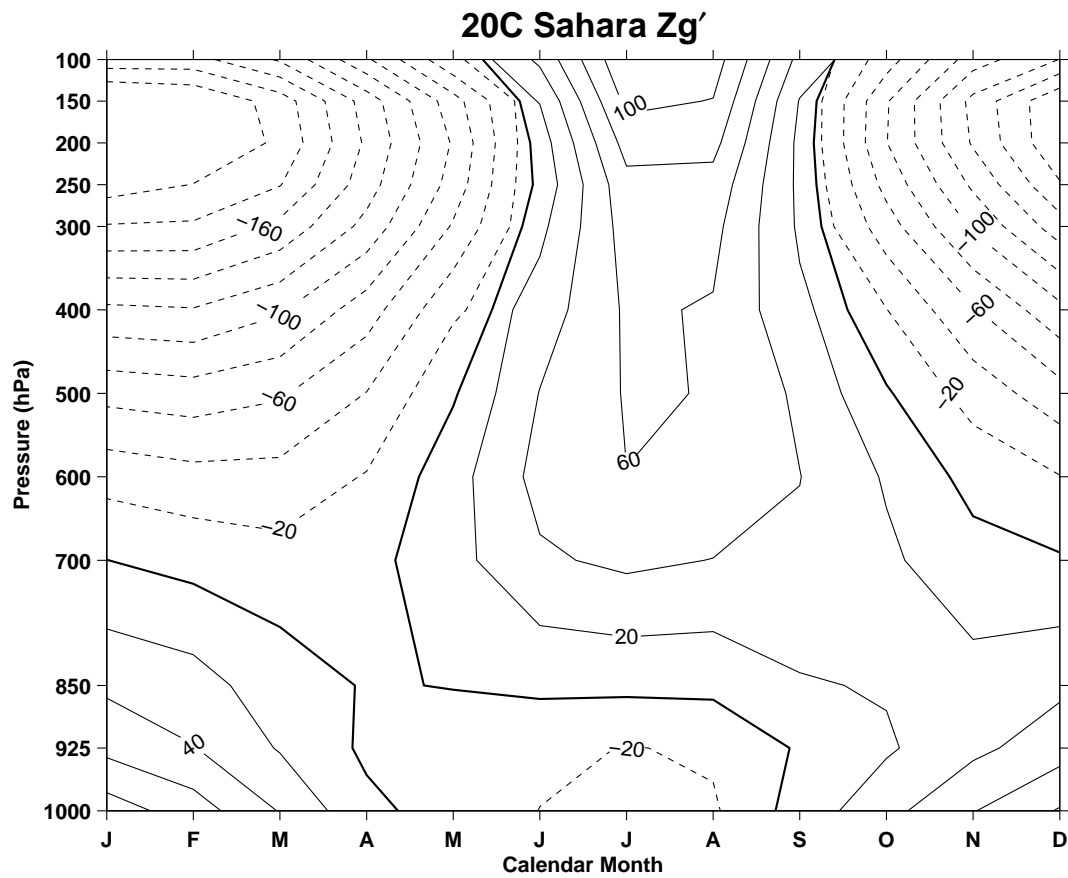
Figure 5. Median annual cycle of 20C Sahara (20N-30N, 10W-35E) mean minus tropical (30S-30N) mean geopotential height, as a function of calendar month and pressure level.
