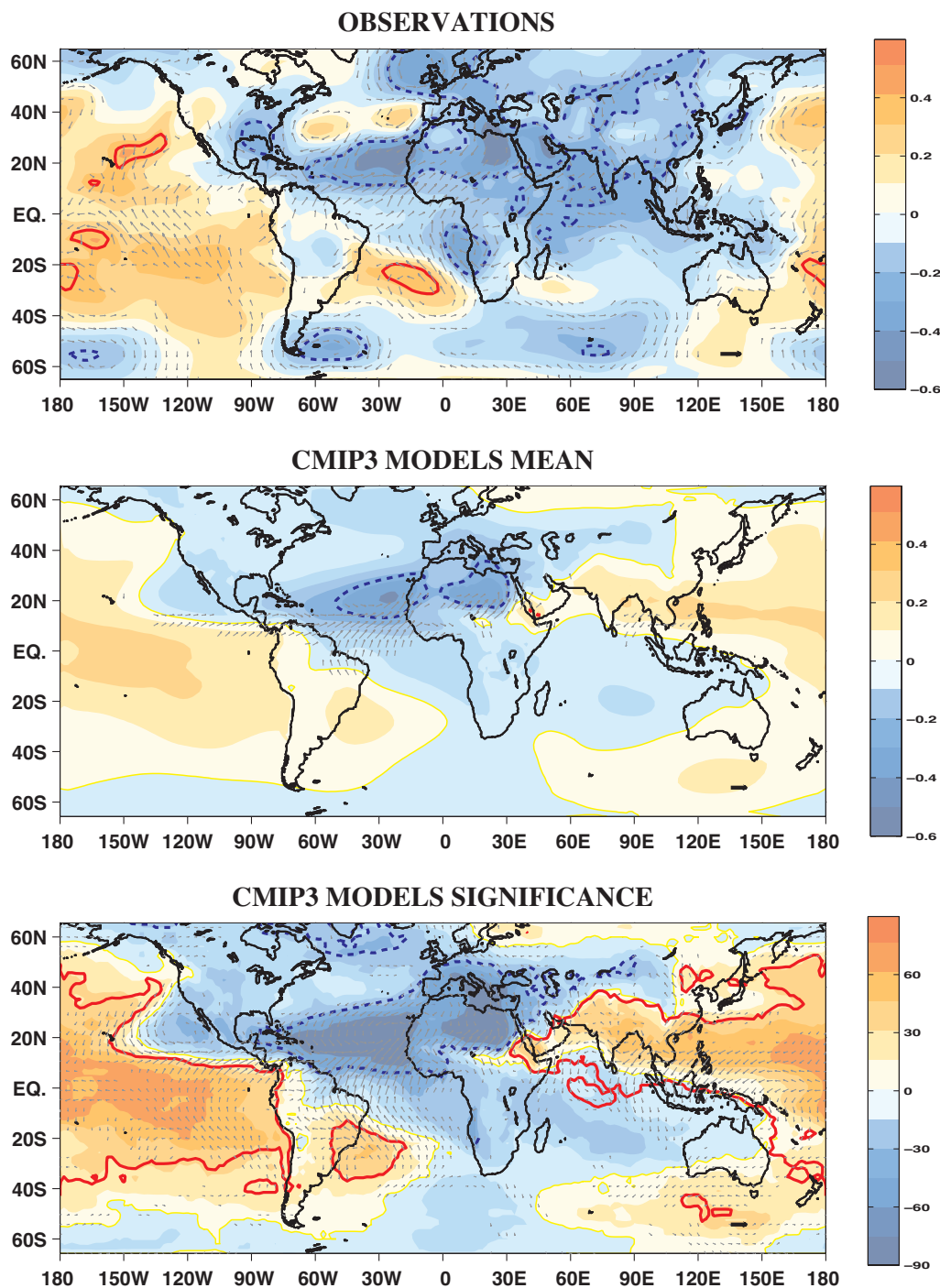
Figure 10. (Top.) Observed correlation between detrended Sahel Index and 925hPa geopotential height (shading interval is 0.1) and winds (westerly and southerly directions indicate positive correlations; only vectors for which at least one component is larger than 0.2 are plotted; the unit vector is plotted in the lower right corner). The thick solid (dashed) contour indicates the 0.3 (-0.3) correlation level with a time series of 925hPa geopotential from which the variability associated with ENSO has been removed. Correlations above \pm 0.21 are significant at the 95% level. (Center.) As in (Top.), but for the CMIP3 mean correlation. (Bottom) Number of models with significant correlation between the detrended Sahel Index and 925hPa geopotential height and winds (units of %; shading interval is 15%; contour is
