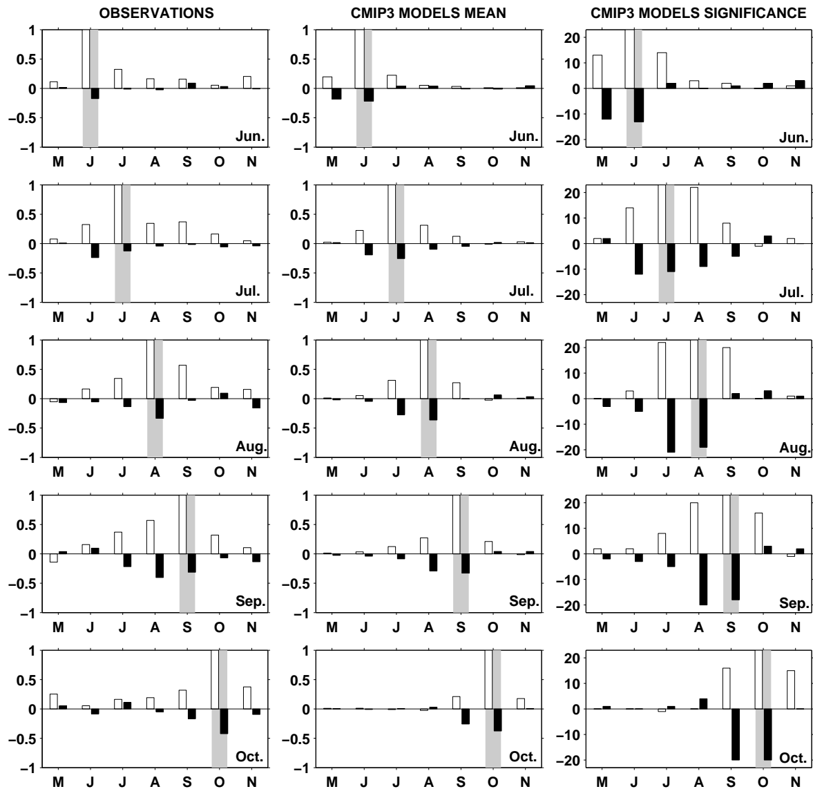
Figure 11. (Left) Observed correlation between detrended Sahel rainfall and sea level pressure over 1900-1998 (Center) Mean CMIP3 correlation and (Right) number of models with significant correlation between the 21C detrended monthly Sahel Index and (open, left bars) itself or (filled, right bars) the Sahara 925hPa geopotential height. In each panel the Sahel index is taken for a different calendar month (June through October, from top to bottom), and the correlations at 0-lag are marked by a grey background.
