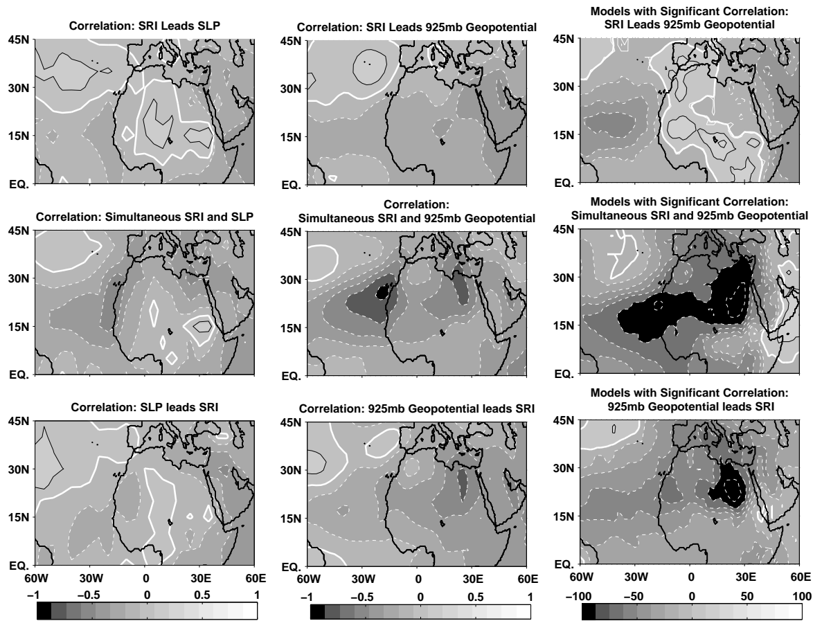
Figure 12. (Left) Observed correlation between detrended August Sahel rainfall and sea level pressure over 1900-1998; (center) correlation of observed Sahel rainfall and the 925hPa geopotential height; (right) number of models (expressed as percentage) with significant (95% level) correlation between the 21C detrended August Sahel Index and 925hPa geopotential height. In the top panels the Sahel index leads (and the geopotential lags) by a month; the middle panels show the 0-lag correlations; the bottom panels show Sahel rainfall lagging by a month. Dark (light) grays and dashed white (solid black) contours indicate negative (positive) correlations, the shading interval is 0.15 for observations and 15% for the models; the zero line is the thick white contour.
