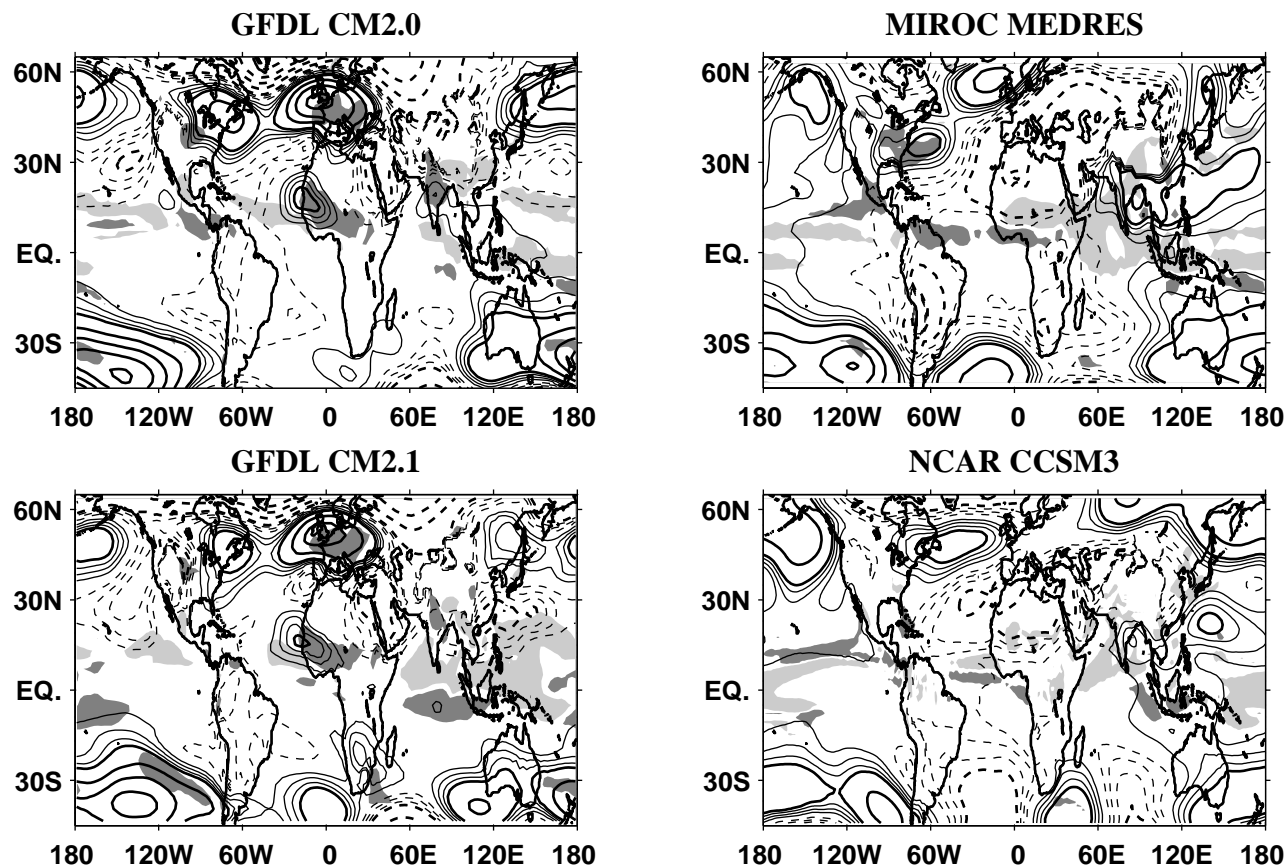
Figure 7. 21C-20C difference in July-August-September 850hPa geopotential height with the tropical mean removed (light lines are \pm 2, \pm 4, \pm 6 , thick lines have a contour interval of 8m) and precipitation [light (dark) shading denotes anomalies greater than positive (negative) 1mm/day].
