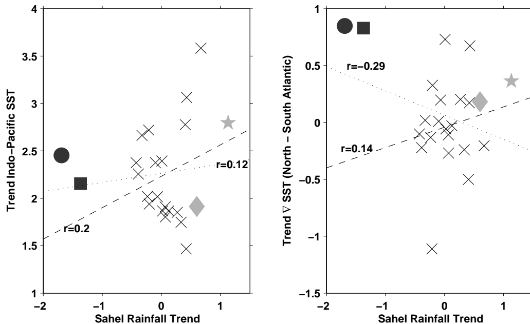
Figure 2. CMIP3 simulations of 21C trend in summer (July-August-September, JAS) Sahel rainfall ( \text{mm day}^{-1} per century) and in (left) tropical Indo-Pacific SST ( 20^{\circ}\text{S} - 20^{\circ}\text{N} ; 50^{\circ}\text{E} - 90^{\circ}\text{W} ; units of ^{\circ}\text{C} per century) and (right) bulk cross-equatorial meridional gradient in tropical Atlantic SST [north ( 7^{\circ}\text{N} - 30^{\circ}\text{N} ; 70^{\circ}\text{W} - 20^{\circ}\text{W} ) minus south ( 20^{\circ}\text{S} - 7^{\circ}\text{N} ; 40^{\circ}\text{W} - 5^{\circ}\text{E} ); units of ^{\circ}\text{C} per century]. The best linear fit lines are calculated using all data (dotted) or excluding four models with extreme anomalies (dashed). The four models are the GFDL CM2.0 (circle) and 2.1 (square), MIROC MEDRES (star) and NCAR CCSM3 (diamond).
