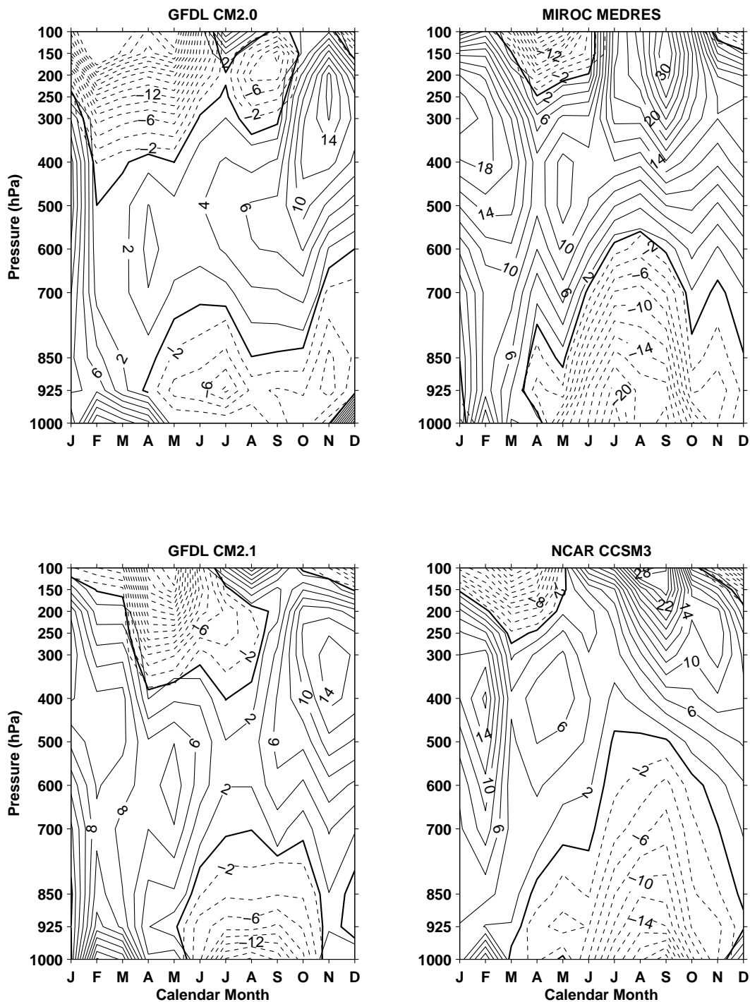
Figure 6. 21C-20C difference in Sahara (20N-30N, 10W-35E) mean minus tropical (30S-30N) mean geopotential height, as a function of calendar month and pressure level in “dry” models (left) and “wet” models (right).
