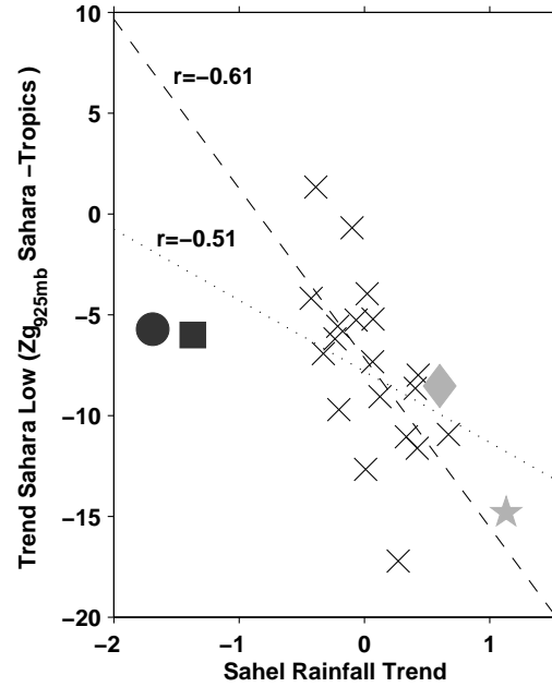
Figure 8. CMIP3 simulations of 21C trend in summer (July-August-September, JAS) Sahel rainfall ( \text{mm day}^{-1} per century) and in the difference in 925hPa geopotential height (meters per century) between the Sahara (20N-30N, 20W-35W) and the tropical band (30S-30N). The best linear fit lines are calculated using all data (dotted) or excluding four models with extreme anomalies (dashed). The four models are the GFDL CM2.0 (circle) and 2.1 (square), MIROC medres (star) and NCAR CCSM3 (diamond).
