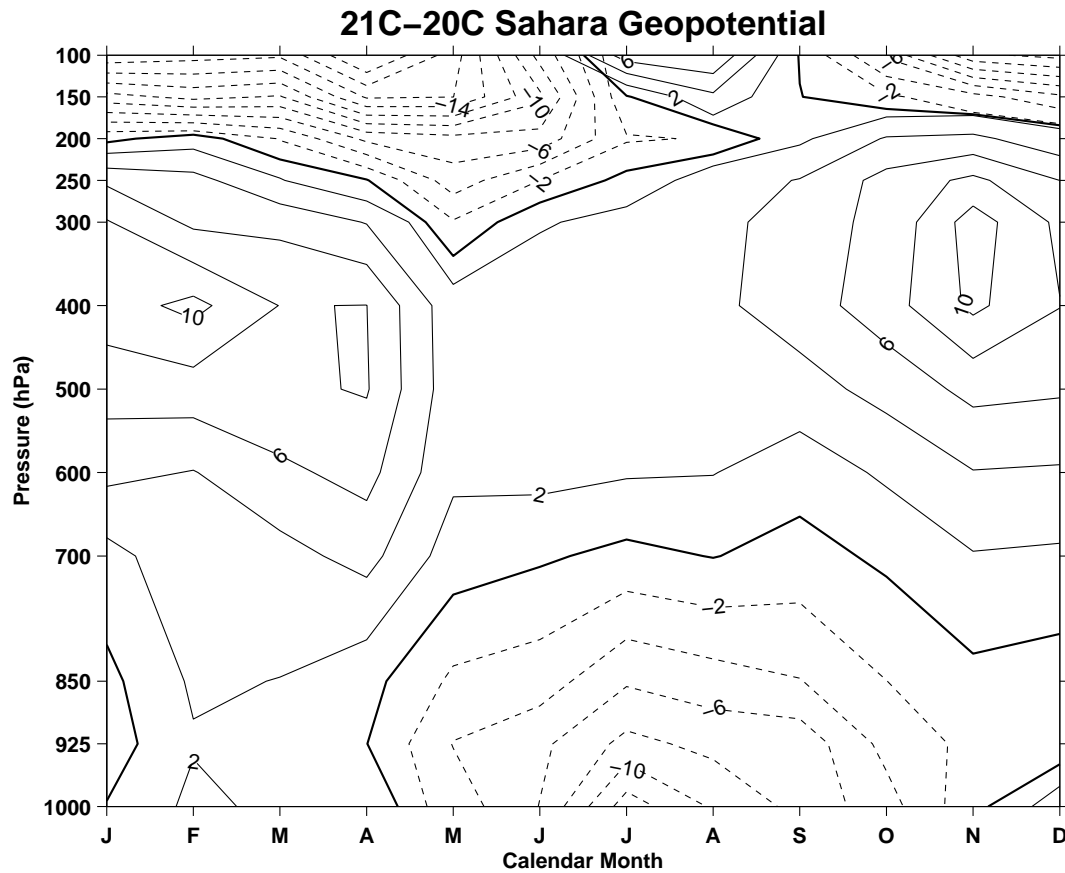
Figure 4. Median 21C-20C difference in Sahara (20N-30N, 10W-35E) mean minus tropical (30S-30N) mean geopotential height, as a function of calendar month and pressure level.
