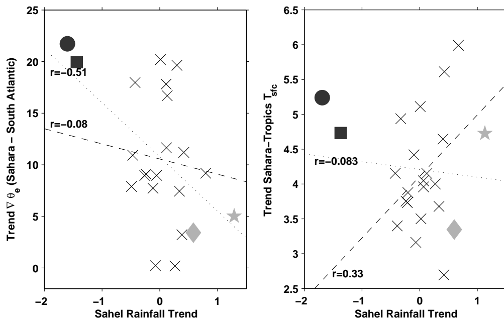
Figure 3. CMIP3 simulations of 21C trend in summer (July-August-September, JAS) Sahel rainfall ( \text{mm day}^{-1} per century) and in (left) bulk meridional gradient in surface equivalent potential energy (K per century) between the Sahara (20N-30N, 20W-35W) and South Tropical Atlantic (20S-Eq., 30W-10E) and (right) surface air temperature ( ^{\circ}\text{C} per century) over the Sahara minus the tropical average (30S-30N). The best linear fit lines are calculated using all data (dotted) or excluding four models with extreme anomalies (dashed). The four models are the GFDL CM2.0 (circle) and 2.1 (square), MIROC MEDRES (star) and NCAR CCSM3 (diamond).
