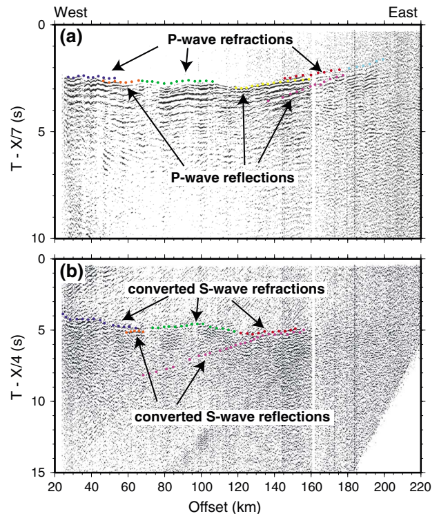
Figure 2. Data from Nikol'ski2 (location in Figure 1). (a) P -wave arrivals in section reduced at 7 km/s. (b) Converted S -wave arrivals in same data reduced at 4 km/s. Refractions from upper (blue), middle (green), lower crust (red), and upper mantle (turquoise). Reflections from base of upper (orange), middle (yellow), and lower crust (purple).
