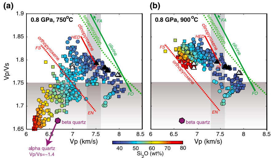
Figure 4. Seismic velocities of obducted arc rocks from Talkeetna and Kohistan [Kelemen et al. , 2003a; Jagoutz et al. , 2006]. Phase proportions and velocities were calculated from bulk composition with a version of Perple_X modified to include the alpha/beta quartz transition at (a) 750°C and (b) 900°C, which lie in the alpha and beta quartz stability fields, respectively. Squares are ultramafic rocks, and circles are gabbros. We assume gabbros contain 0.5 wt % H 2 O and ultramafic rocks are dry. Grey, black, and white triangles are velocities estimated for (olivine-) pyroxenites, dunites, and other compositions (amphibolites and hornblendites) from Aleutian xenoliths, respectively [DeBari et al. , 1987] using Hacker and Abers [2004]. Grey bands show range of V_P from Shillington et al. [2004] and V_P/V_S from this study. Lines and text indicate V_P and V_P/V_S for compositional end-members of olivine (FO-fosterite, FA-fayalite), clinopyroxene (DI-diopside, HED-hedenbergite), and orthopyroxene (EN-enstatite, FS-ferrosillite) from Hacker and Abers [2004]. Serpentinite calculated at 600°C. Almost no compositions fall within observed V_P and V_P/V_S ranges for the Aleutian lower crust, suggesting that a mixture of compositions is required.
