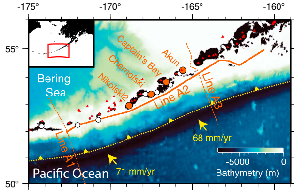
Figure 1. Map with 1994 Aleutian experiment. Bold orange line shows shotline used in this study. Instruments shown with white circles; instruments whose data are used here shown with orange circles and text. Red triangles indicate volcanoes from the Smithsonian Global Volcanism Program. Plate boundary and convergence directions and rates with respect to North American shown with yellow dotted lines, arrows and text [DeMets et al. , 2010].
