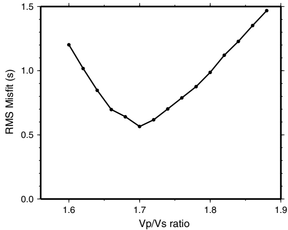
Figure 3. RMS residuals for various lower crustal V_P/V_S for S -arrivals on instruments shown in Figure 1.
