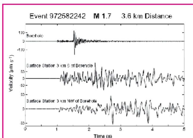
Figure 1. Comparison of vertical component seismograms recorded in LVEW (Long Valley Exploratory Well) at a depth of 2050 m with vertical records from two conventional surface seismic stations located near the borehole. Note the impulsive nature of the P- and S- wave arrivals, the high frequency content, and relative lack of scattering in the coda in the borehole records with respect to the surface records (from Prejean and Ellsworth, 2001).
