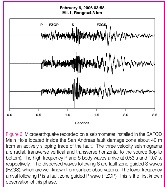
Figure 6. Microearthquake recorded on a seismometer installed in the SAFOD Main Hole located inside the San Andreas fault damage zone about 40 m from an actively slipping trace of the fault. The three velocity seismograms are radial, transverse vertical and transverse horizontal to the source (top to bottom). The high frequency P and S body waves arrive at 0.53 s and 1.07 s, respectively. The dispersed waves following S are fault zone guided S waves (FZGS), which are well-known from surface observations. The lower frequency arrival following P is a fault zone guided P wave (FZGP). This is the first known observation of this phase.
