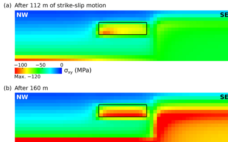
Fig. 7. Along-strike shear stress map on the fault plane at two stages of the simulation (after 112 and 160 m of displacement). Note the x axis is into the plane and the y axis is pointing to the left. So, the right-lateral motion generates negative values of shear stress ( \sigma_{xy} ).
