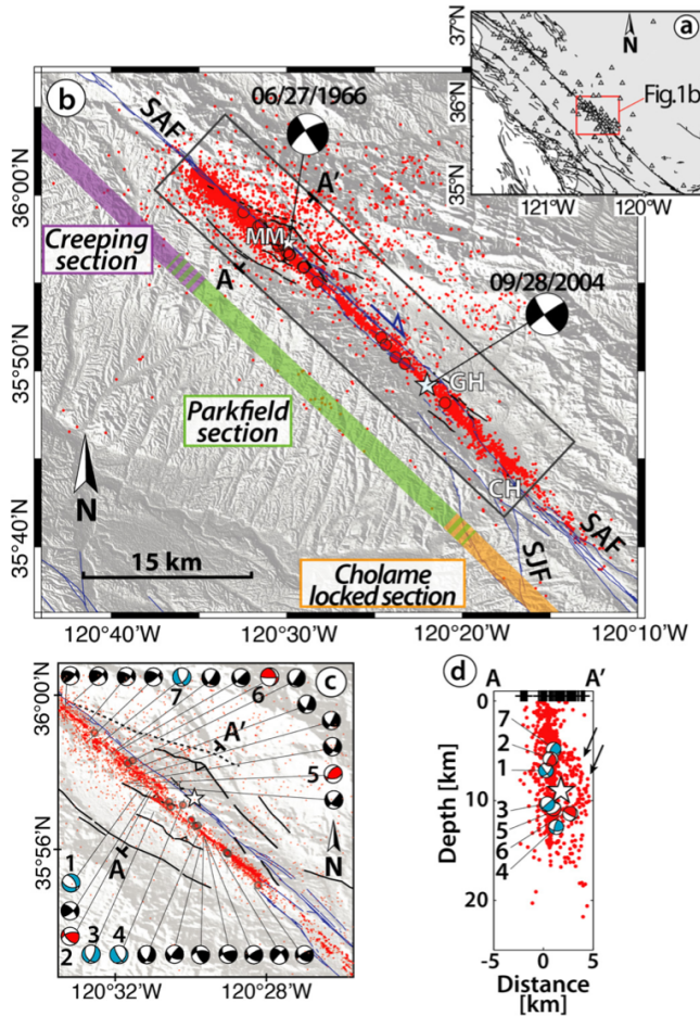
Fig. 1. a) Map view of central California. White triangles are the 212 stations that recorded the ~17,000 events; b) Fault map along the Parkfield section and relocated seismicity (red dots) from 1966 to 2015. Black circles are events with M \geq 4 . White stars are the 1966 and 2004 epicenters. Fault traces are shown on SRTM3 topography illuminated from the southwest. Blue lines are quaternary fault traces from the (U.S. Geological Survey and California Geological Survey, 2006); black lines are additional long-term fault traces from this study and Thayer (2006) (dotted black lines when uncertain). SAF: San Andreas Fault; SJF: San Juan Fault; MM: Middle Mountain; GH: Gold Hill; CH: Cholame; c) Zoom into Middle Mountain area. Focal mechanisms (Hardebeck, 2010) showing intermediate to low-angle dipping fault motions ( < 70^\circ ). d) Cross section (AA') showing the relocated seismicity from 1966 to 2015 (red dots) at Middle Mountain. Black crosses are fault traces at surface. The white star represents the 1966 hypocenter. Black arrows point possible secondary active strands at depth. Numbered focal mechanisms in c) and d) point out specific thrust (red) and normal (blue) faulting earthquakes (front projection). (For interpretation of the colors in the figure(s), the reader is referred to the web version of this article.)
