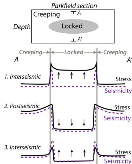
Fig. 9. Sketch showing a simplified view of the Parkfield fault section and along dip distribution of stress and seismicity rates (profile AA') as predicted from a locked patch at mid-crustal depth imbedded in an otherwise creeping fault. Seismic activity is driven by the difference in the stress rate at the edge of the locked patch at every stage of the earthquake cycle.
