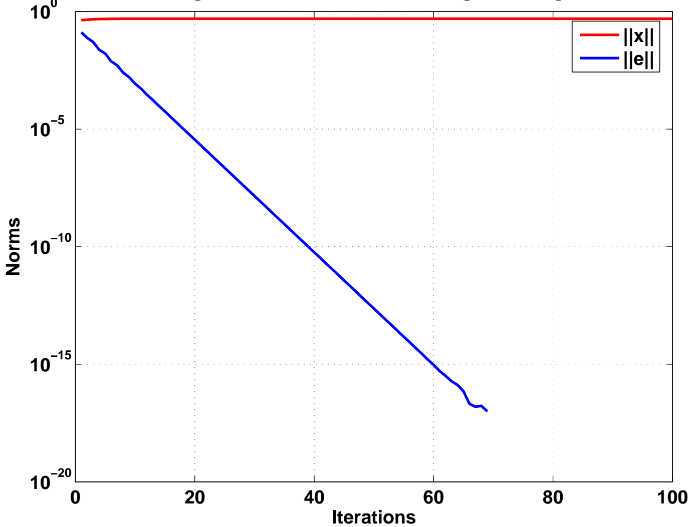
Convergence of Power method for PageRank Algorithm
