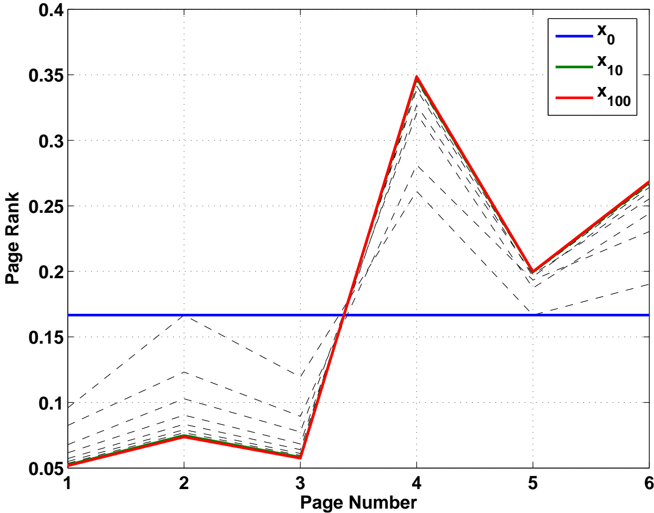
Evolution of PageRank probability
