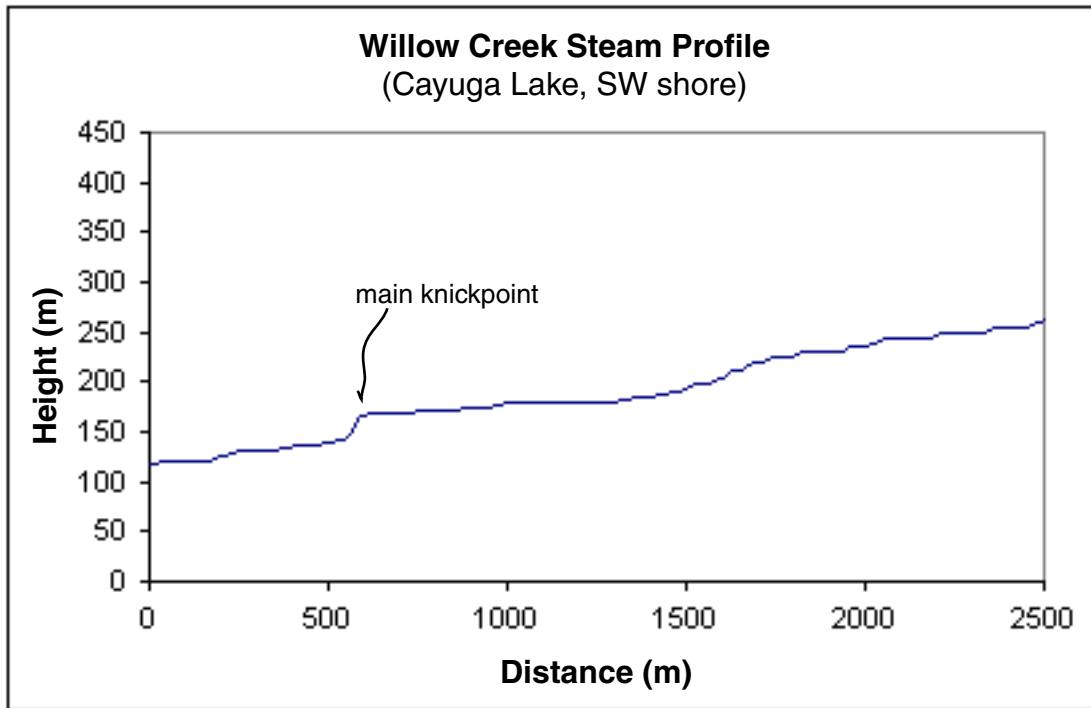
Figure 1. Profile of Willow Creek (Ludlowville and Ithaca West Quadrangles), showing a major knickpoint along the profile (height ~ 15 m). Other knickpoints are present along the stream, but are smaller in magnitude.
