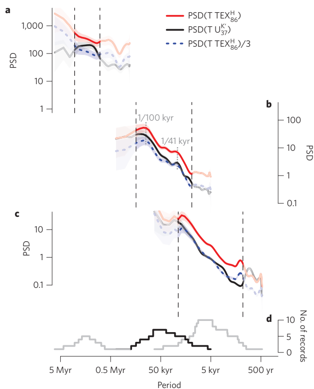
Figure 1 | Spectral estimates of U_{37}^{K'} - and TEX_{86}^H -inferred temperature variability. a–c , Mean power spectral density (PSD) estimate of the globally distributed single records for three time intervals: multi-million years ( a ), past one million years ( b ), last glacial cycle ( c ). d , Number of records contributing to each frequency. Dividing the TEX_{86}^H -inferred variability by three (dashed blue line) results in a spectral estimate similar to that derived from U_{37}^{K'} SST. As averaging across records is needed to damp the effect of regionally differing surface and subsurface variability (Supplementary Fig. 3), estimates based on fewer than three records are shaded white. Proxy records constituting the composite spectra are listed in Supplementary Fig. 2. Shading indicates 95% confidence intervals representing the uncertainty of the spectral estimate.
