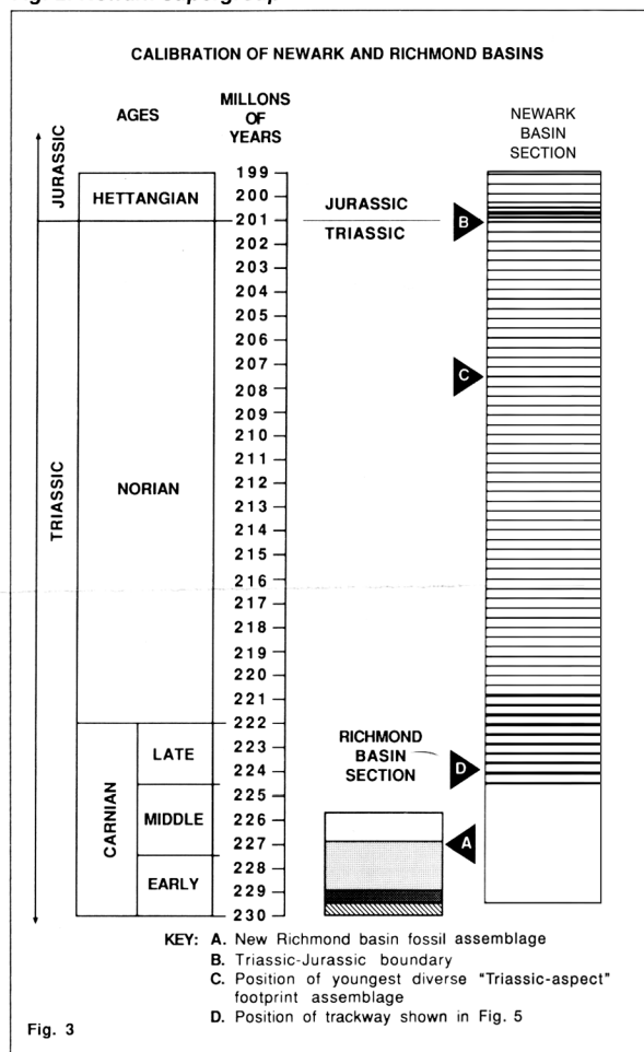
Fig. 3: Use of lake level cycles has allowed a fine-scale time calibration of the stratigraphic sections in the Newark and Richmond basins. Ages are the paleontologically defined time divisions of the Early Mesozoic. Time in millions of years is based on lake level cycles (400,000 year cycle) shown as horizontal bars in the Newark basin section.
