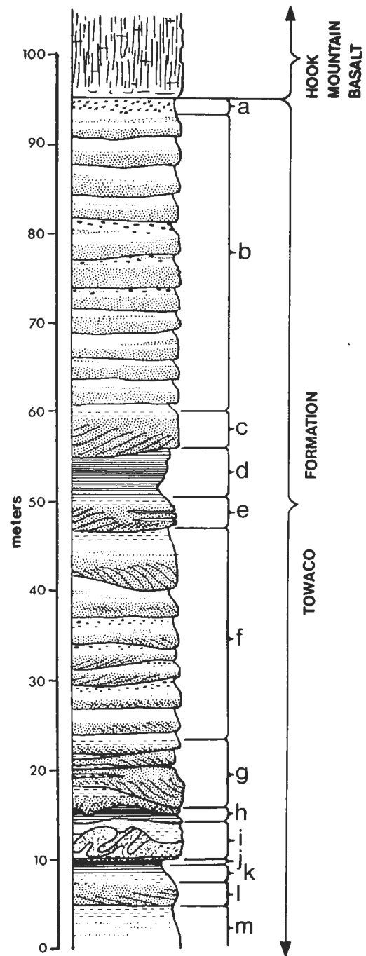
Fig. 10 Type section of the Towaco Formation in the Dinosaur Tract, Essex County Park Commission, Roseland, New Jersey. For key to individual units.
