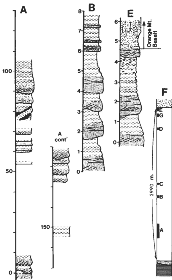
Fig. 4 A - E, type section of Passaic Formation (Table 5 for description); F, diagram showing positions of sections A - E in Passaic Formation.
