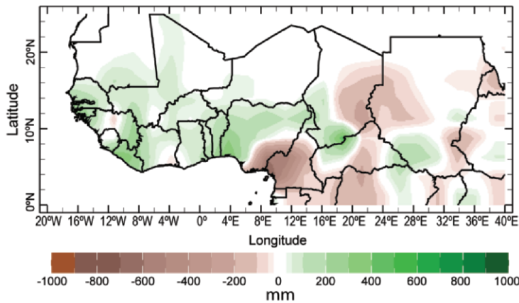
FIG. 7.17. May to Oct 2008 accumulated precipitation anomalies (mm) for western Africa (1971–2000 reference period). (Source: GPCP, Version 2 Monitoring Product.)
