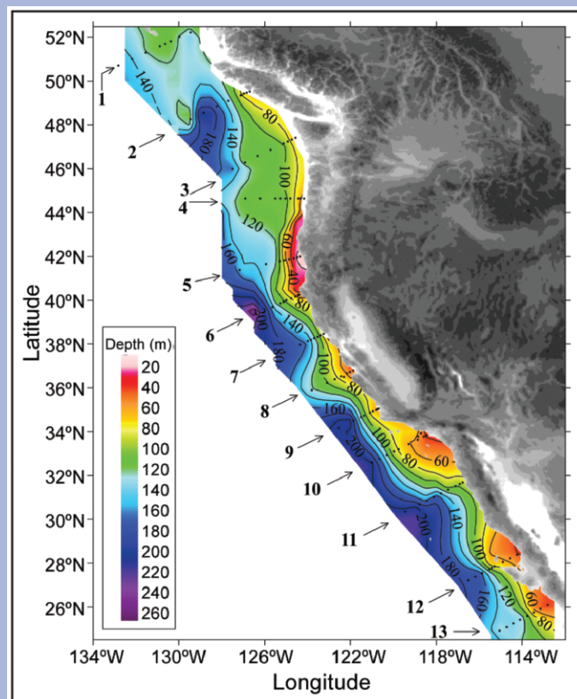
FIG. 3.29 (after Feely et al. 2008). Distribution of the depths of “ocean acidified” undersaturated water (aragonite saturation <1.0 ; \text{pH} < 7.75 ) on the continental shelf of western North America from Queen Charlotte Sound, Canada, to San Gregorio Baja California Sur, Mexico. On transect line 5, the corrosive water reaches all the way to the surface in the inshore waters near the coast. The black dots represent station locations.
