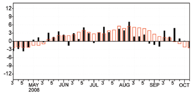
FIG. 7.39. Variation of pentad zonal wind index over monitoring region (10°–20°N, 110°–120°E), red open bars stand for climatology (Unit: m s^{-1} ) (Source: CMA.)
