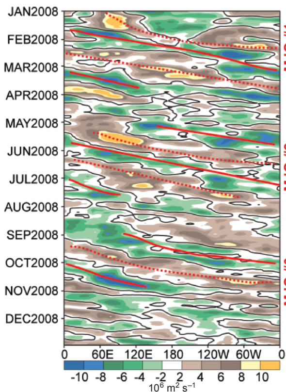
FIG. 4.6. Time–longitude section of filtered 200-hPa velocity potential anomaly ( 5^{\circ}\text{N} – 5^{\circ}\text{S} ) for 2008. Green (brown) shading represents anomalous divergence (convergence). Red lines highlight the MJO signal. The three MJO episodes are marked. Anomalies are departures from the 1971–2000 base period daily means.
