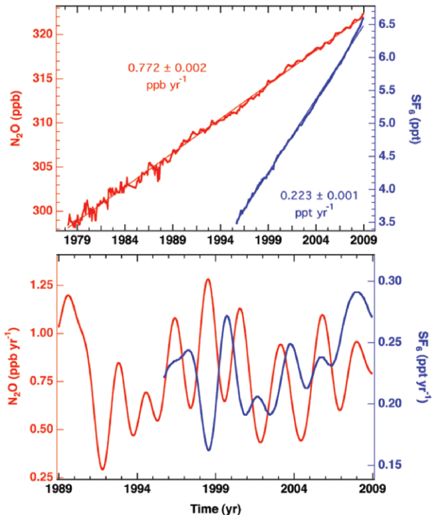
FIG. 2.31. (top) Global monthly means along with estimates for the linear growth rate of atmospheric nitrous oxide (N 2 O, red) in ppb and sulfur hexafluoride (SF 6 , blue) in ppt from the NOAA/ESRL halocarbon network. (bottom) Instantaneous growth rate of N 2 O and SF 6 using a smoothing algorithm with a 2-yr filter; note the rapid rise of the atmospheric SF 6 growth rate after 2003. Atmospheric data for N 2 O prior to 1989 and for SF 6 prior to 1999 were analyzed from flasks instead of continuously operating instruments at NOAA/ESRL baseline observatories.
