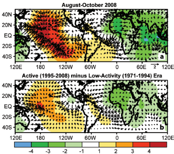
FIG. 4.12. 200-hPa velocity potential (shading) and divergent wind vectors ( \text{m s}^{-1} ): (a) Aug–Oct 2008 anomalies and (b) high-activity (1995–2008) period means minus low-activity (1971–94) period means. Anomalies are departures from the 1971–2000 monthly means.
