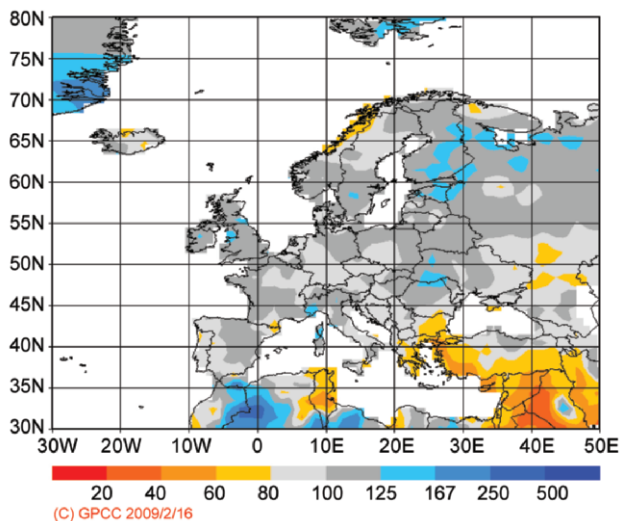
FIG. 7.26. European precipitation totals (percentages of normal, 1951–2000 base period) for the whole year 2008. (Source: GPCC; Rudolf et al. 2005.)
