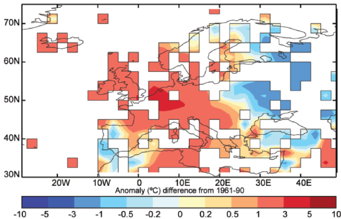
FIG. 7.28. May 2008 mean temperature anomalies in Europe, ( ^{\circ}\text{C} , 1961–90 base period), based on CRUTEM3 dataset (Source: Brohan et al. 2006).
