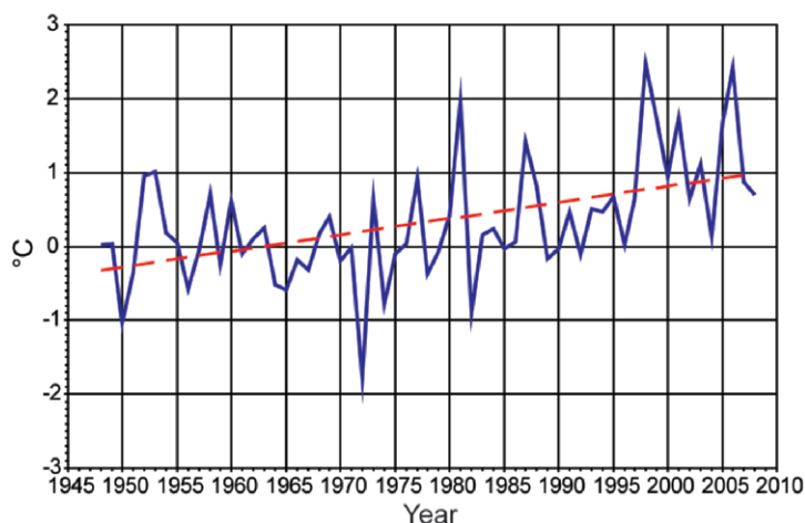
FIG. 7.1. Annual mean temperature anomalies for Canada, 1948–2008. (Source: Environment Canada.)
