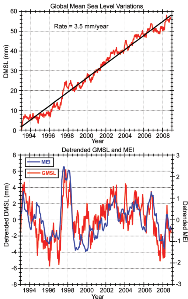
FIG. 3.22. (top) Monthly GMSL (seasonal cycle removed) relative to a linear trend of 3.5 mm yr -1 . (bottom) Monthly GMSL (linear trend removed, red) versus the MEI (blue). SSH data provided by the NASA PO.DAAC at the Jet Propulsion Laboratory/California Institute of Technology ( http://podaac.jpl.nasa.gov/ ).
