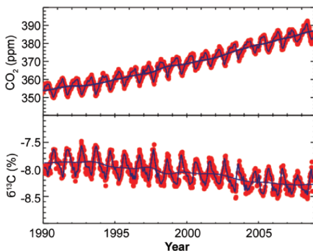
FIG. 2.27. \text{CO}_2 dry air mole fractions (top: NOAA ESRL) and \delta^{13}\text{C} in \text{CO}_2 (bottom: University of Colorado, INSTAAR, courtesy James White) from weekly samples at Cape Kumukahi, HI.
