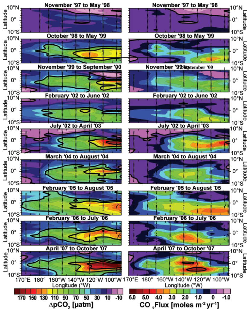
FIG. 3.25. Plots of sea-air p\text{CO}_2 difference and air-sea \text{CO}_2 flux in the equatorial Pacific between 1997 and 2007 based on underway \text{CO}_2 measurements collected on the TAO service cruises. The nominal cruise track lines are shown in black. A complete survey of the region is completed approximately every six months. The black and dark purple areas indicate where the atmosphere and seawater p\text{CO}_2 values are nearly balanced. The pink areas indicate ocean uptake of \text{CO}_2 , and the blue to red colors indicate areas of ocean \text{CO}_2 out-gassing.
