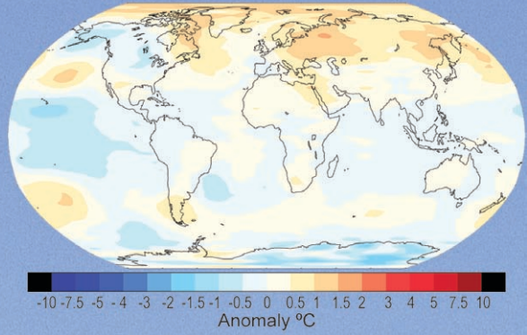
Lower stratospheric temperature
