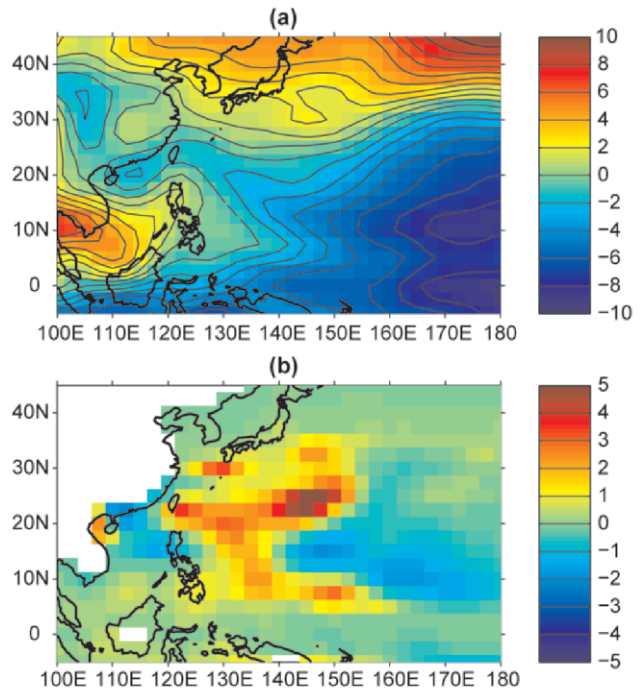
FIG. 4.20. (a) Zonal 850-hPa winds ( \text{m s}^{-1} ) from JASO 2008. The contour interval is 1 \text{ m s}^{-1} . (b) Genesis potential index (Camargo et al. 2007b) anomalies for JASO 2008. (Source: atmospheric variables—NCEP reanalysis data; Kalnay et al. 1996; SST—Smith and Reynolds 2005.)
