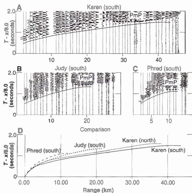
Fig. 2. (A through C) Travel time ( T ) versus range ( X ) plots of seismic data for OBSs Karen (A), Judy (B), and Phred (C). The solid lines are cubic spline fits to the initial P -wave arrival picks. The thick dashed line shows the area of high amplitude associated with the PmP arrival; the north-south labels indicate which side of the instrument the shots were on. The data are plotted with a reduction velocity of 8 km/s. Corrections for along-axis variations in topography were estimated by locating the least time entry point on the sea floor and subtracting the associated travel time to this entry point from the shot time (30). The data picks were then smoothed by fitting a cubic spline constrained to be monotonically decreasing in slope to permit a \tau - p (where \tau is delay time and p is the ray parameter) inversion for a smooth velocity-depth model (31). (D) A comparison of the cubic spline fits for four record sections on the 33°S segment.
