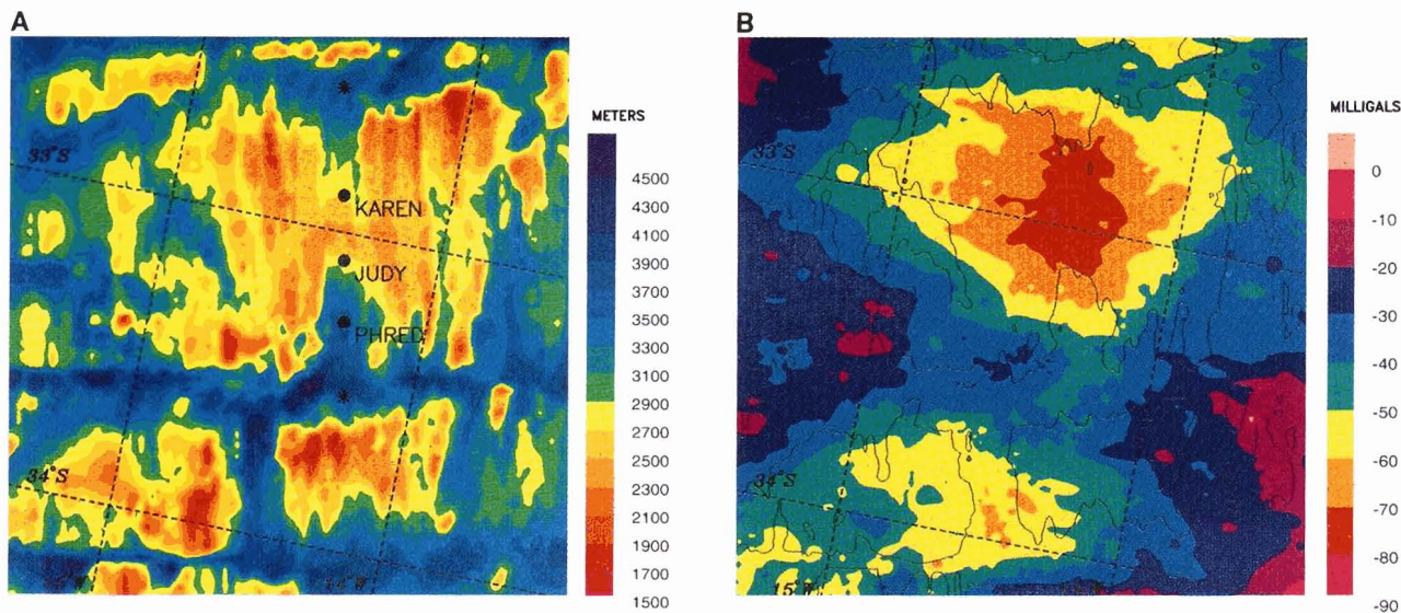
Fig. 1. (A) Bathymetry map of the 33°S segment of the southern MAR (2). Circles mark locations of OBSs and asterisks indicate the start and end points (bottom and top, respectively) of the shot line. (B) Mantle Bouguer
