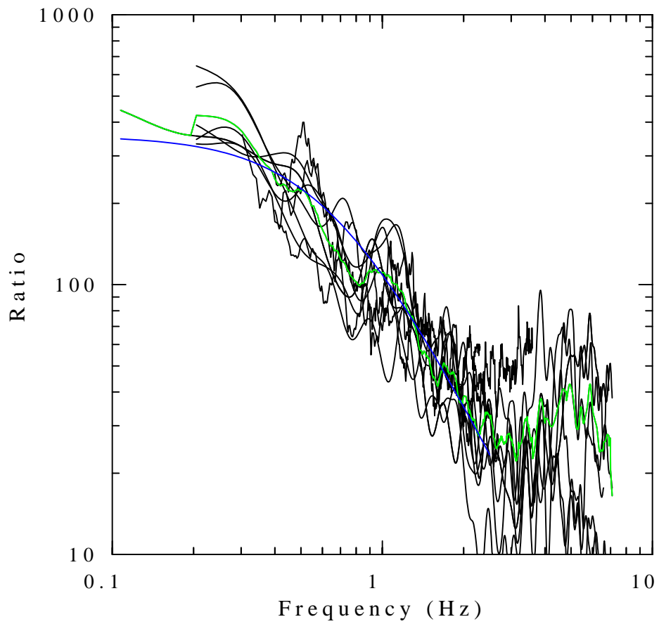
Spectral ratios at 16 stations, 041197/041497
