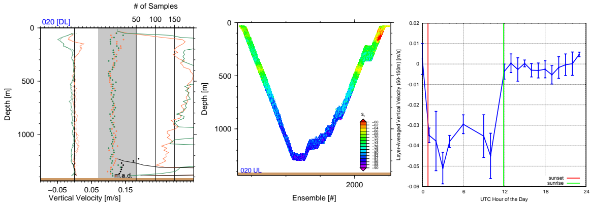
Figure 15: Upper-ocean vertical velocity signals in the northeastern Gulf of Mexico likely caused by biology; software V1.2. Left and middle panels: Diagnostic w_{prof} and backscatter plots from an example profile with strong apparent downwelling observed during the upcast in the upper 200 m of the water column. Right panel: Average w_{ocean} between 50 and 150 m vs. hour of the day for all profiles from this site.
