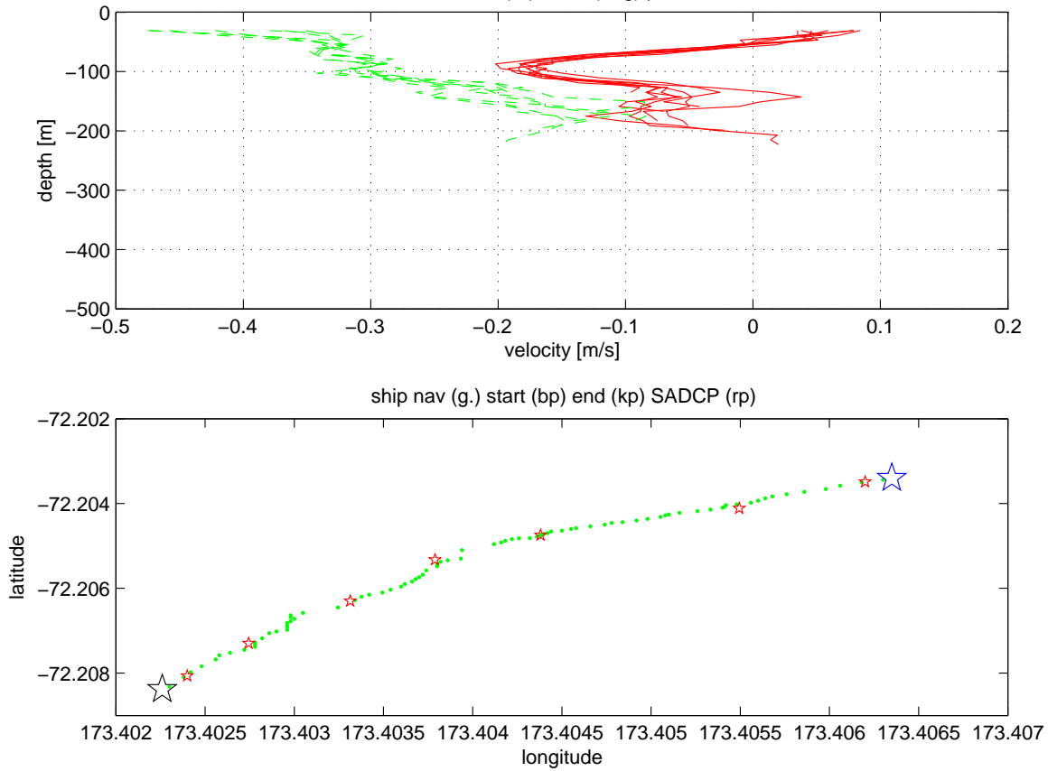
ProcFig. 9: SADCPC data. Upper panel: Ensemble of ADCP velocity profiles in time-range of cast. Lower panel: Ship track from GPS (blue stars and green dots) and location of SADCPC profiles (red stars).
