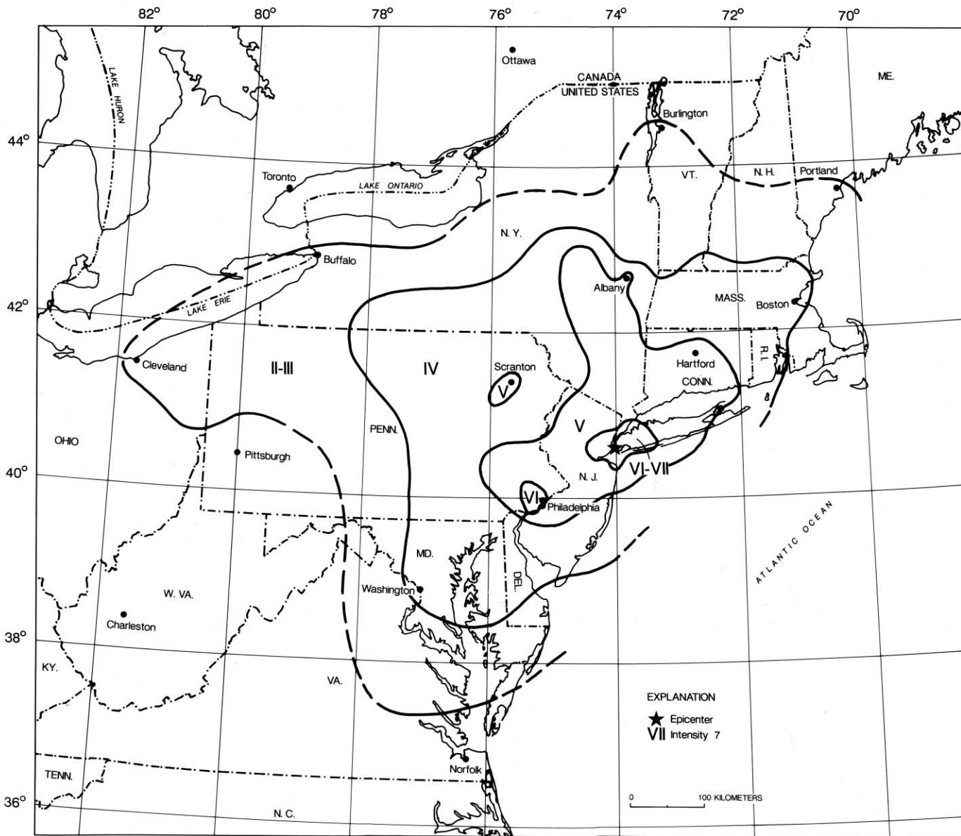
FIGURE 46.— Isoseismal map for the New York City, New York, earthquake of August 10, 1884. Isoseismals are based on intensity estimates from data listed in references 369, 463, 518, and 529 of table 1.
