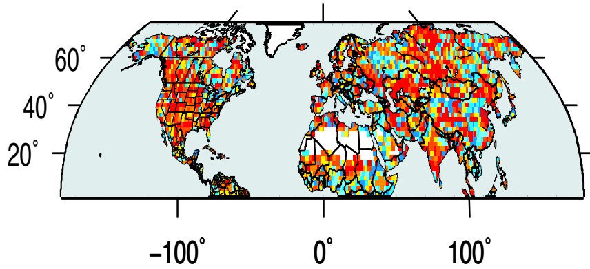
Cross-Validation R^2
