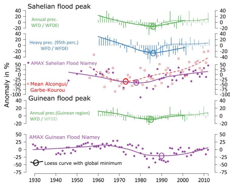
Figure 5. Sahel Paradox depicted with annual/ heavy precipitation from WFD and WFDEI and AMAX for the Sahelian flood peak at Niamey, and the mean of Alcongui and Garbe-Kourou. The AMAX of the Guinean flood peak at Niamey is depicted with the respective precipitation in order to illustrate the difference. All time series as anomalies in % with Loess curves and global minima.
