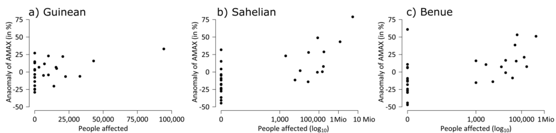
Figure 9. Correlation between AMAX and people affected by floods for the subregions of the Niger basin, (a) Guinean, (b) Sahelian and (c) Benue. The scales for people affected by floods for the Sahelian region and the Benue are logarithmic. Please note that the number of people affected for the Sahelian basin comprises the whole Middle Niger (See Section 3.1.2).
