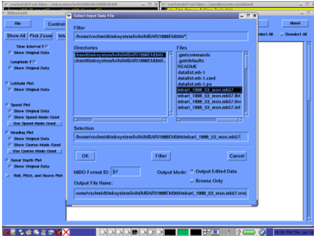
Figure 4.17. MBnavedit
