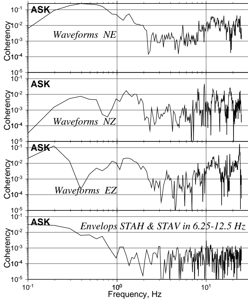
Fig. 4. Observed noise coherence between 3-component waveforms and STAH and STAV envelopes. This is original noise waveforms recorded by our novel ASK station of length 60 min presumably free of signals. Coherency at levels of 0.01 or less give component independency for the ambient noise field. Also note that similar results were obtained when noise waveforms were replaced by the corresponding envelopes, in this case the coherency is less than 0.001. In the STA/LTA 2D detector the test statistics are the noise and signal envelopes.
