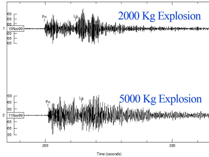
Comparison of EIL Vertical Recordings for Two Events - PIDC Phase Picks
