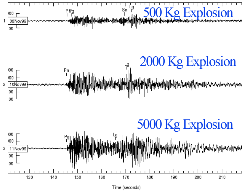
Comparison of MRNI Vertical Recordings for Three Events - PIDC Phase Picks
