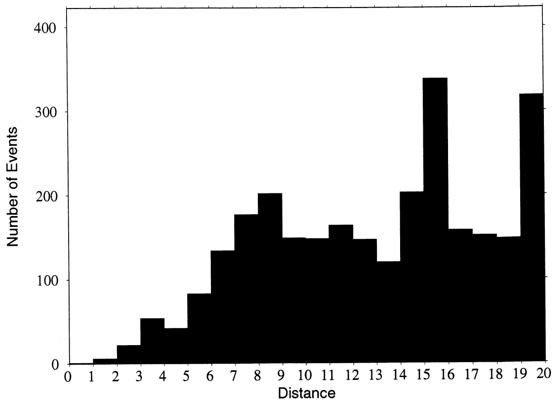
Figure 5. Distributions with respect to epicentral distance of the regional events with Lg signals reported at CMAR (top) and a large sample of 2767 REB events within 20° of CMAR (bottom) from which supplemental data have been selected.
