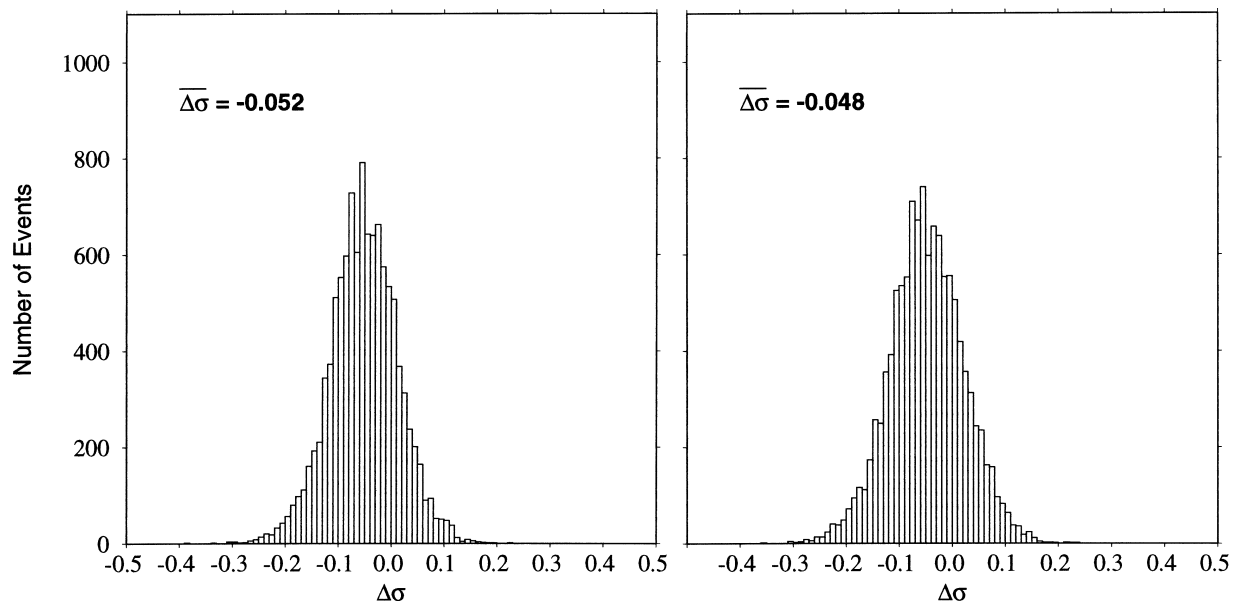
Figure 3. Comparison of the observed reductions in the standard errors of estimate obtained by applying the station corrections to all the single station P wave data in the distance range from 25 to 180 degrees (left) with those obtained for the distance range from 25 to 100 degrees (right).
