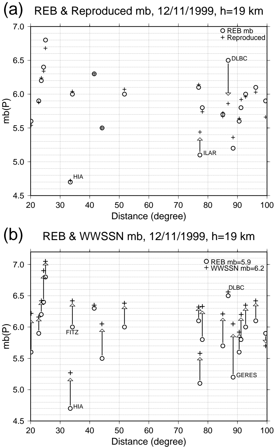
Figure 5. (a) Comparison m_b s reported by REB ( circles ) and reproduced in this study ( plus ). Notice that reproduced m_b at ILAR is about 0.3 m.u. greater than REB m_b , whereas at DLBC reproduced m_b is 0.6 m.u. smaller than REB m_b , (b) Comparison of the station m_b (VC) and m_b (REB). Arrows indicate sign and size of the m_b (REB) - m_b (VC). The average difference between these two magnitudes is 0.33 m.u.
