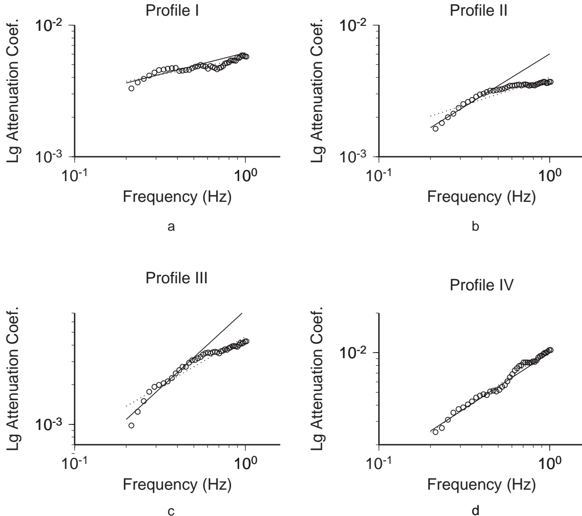
Figure 5. L_g attenuation coefficient g(f) and the best fit Q_{Lg} models (straight lines) for each profile. Circles are mean values estimated from stacking multiple spectral ratios in each profile. Solid and dashed lines represent the best fit Q_{Lg} models in frequency bands of 0.2-0.5 Hz and 0.2-1.0 Hz, respectively.
