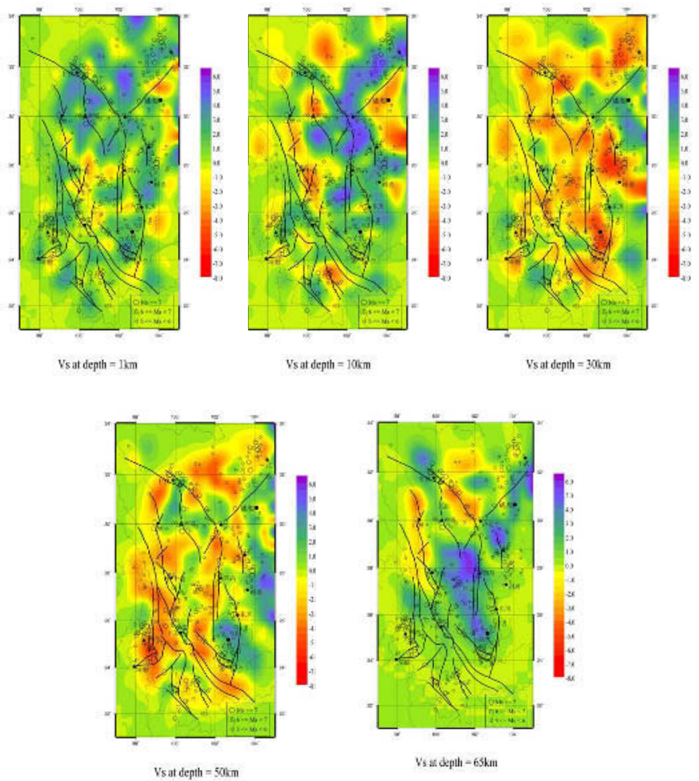
Figure 9. Tomographic inversion results for S waves
