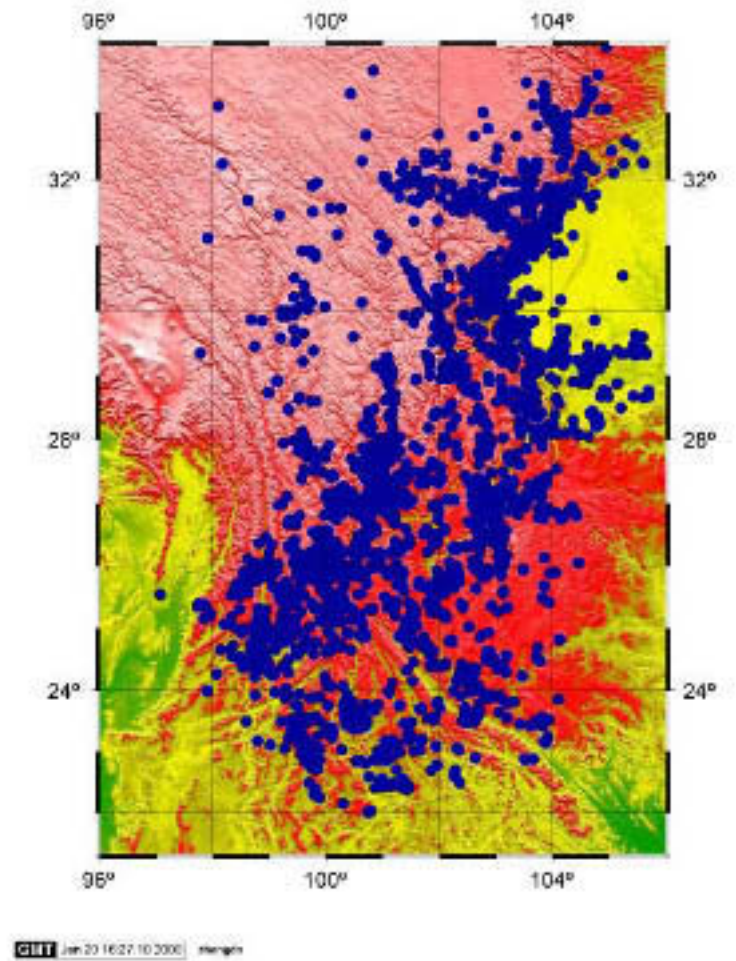
Figure 5. Earthquake distribution in the SYR
