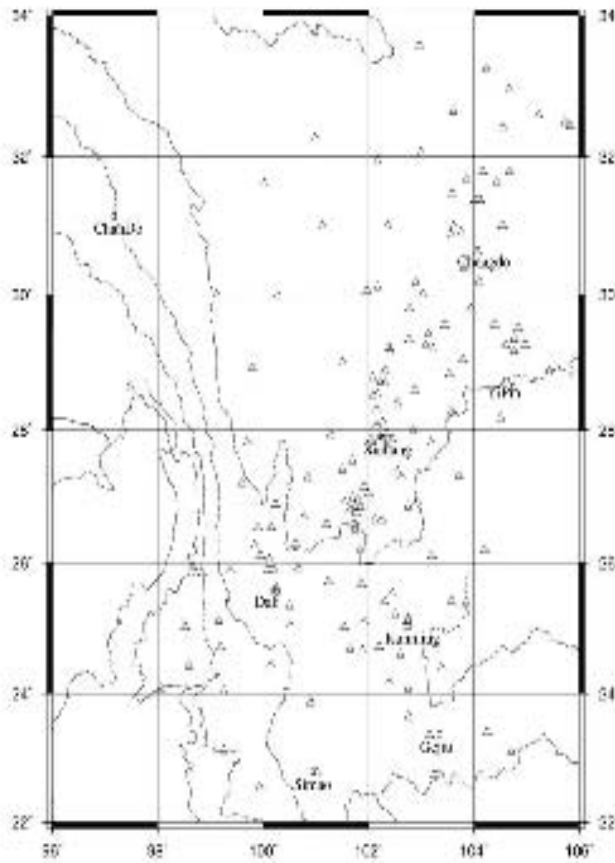
Figure 4. Station locations in SYR
