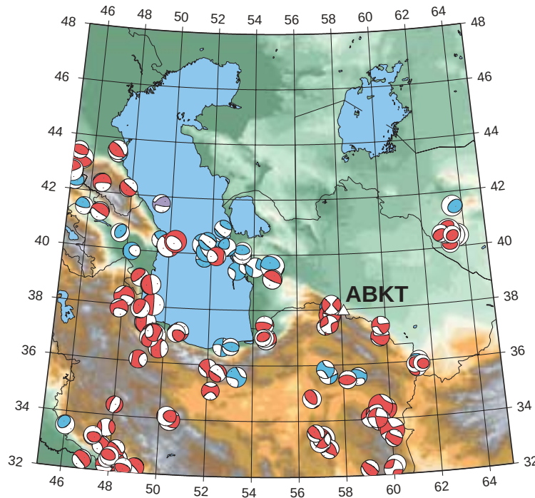
Figure 2. Location of station ABKTat Alibek, Turkmenistan (37.9304N, 58.1189E, 678 m), shown with topographic variations and focal mechanisms from the Harvard CMT catalog. Mechanisms are shaded by depth (red indicated depths from 0 to 32 km; blue depths from 33 to 70 km; and purple depths greater than 70 km).
