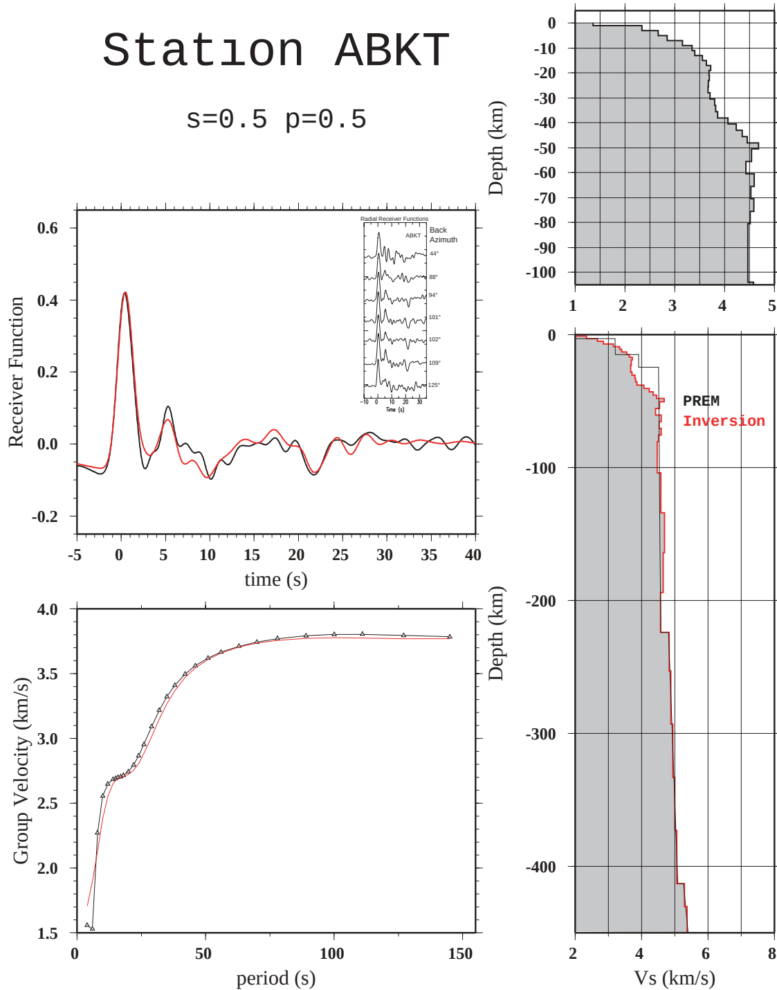
Figure 4. Inversion results for station ABKT using Stevens' dispersion model and a receiver function appropriate for the region east-northeast of the station. Red lines identify predictions, black lines (and symbols) the observations. The subset of receiver functions used to compute the stack used in the inversion is shown in the inset of the upper left panel. The gray shaded models is the result of the inversion.
