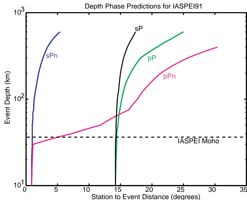
Figure 5. Depth phase arrivals at regional and near-teleseismic distances as a function of epicentral distance and event depth. The plot shows the initial distance from an event in which a depth phase (either pPn , sPn , pP , or sP ) is theoretically predicted to occur from IASPEI91 (Kennett and Engdahl, 1991) as a function of the event depth. For the near-regional analysis ( < 10^\circ ) of the AEIC data, we can only detect sPn and pPn phases for crustal events ( < 35 km), while deeper events may only have the sPn arrival.
