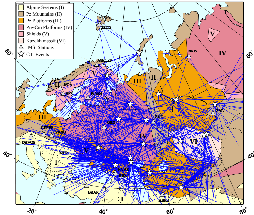
Figure 1. Calibration events used for development of 3-D velocity models. Lines are Pn event-station paths.
