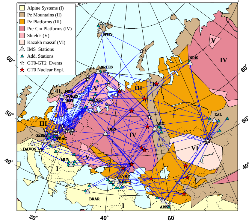
Figure 5. GT events used for relocation experiments. Lines connect the events with seismic stations used for relocation experiments at regional distances.
