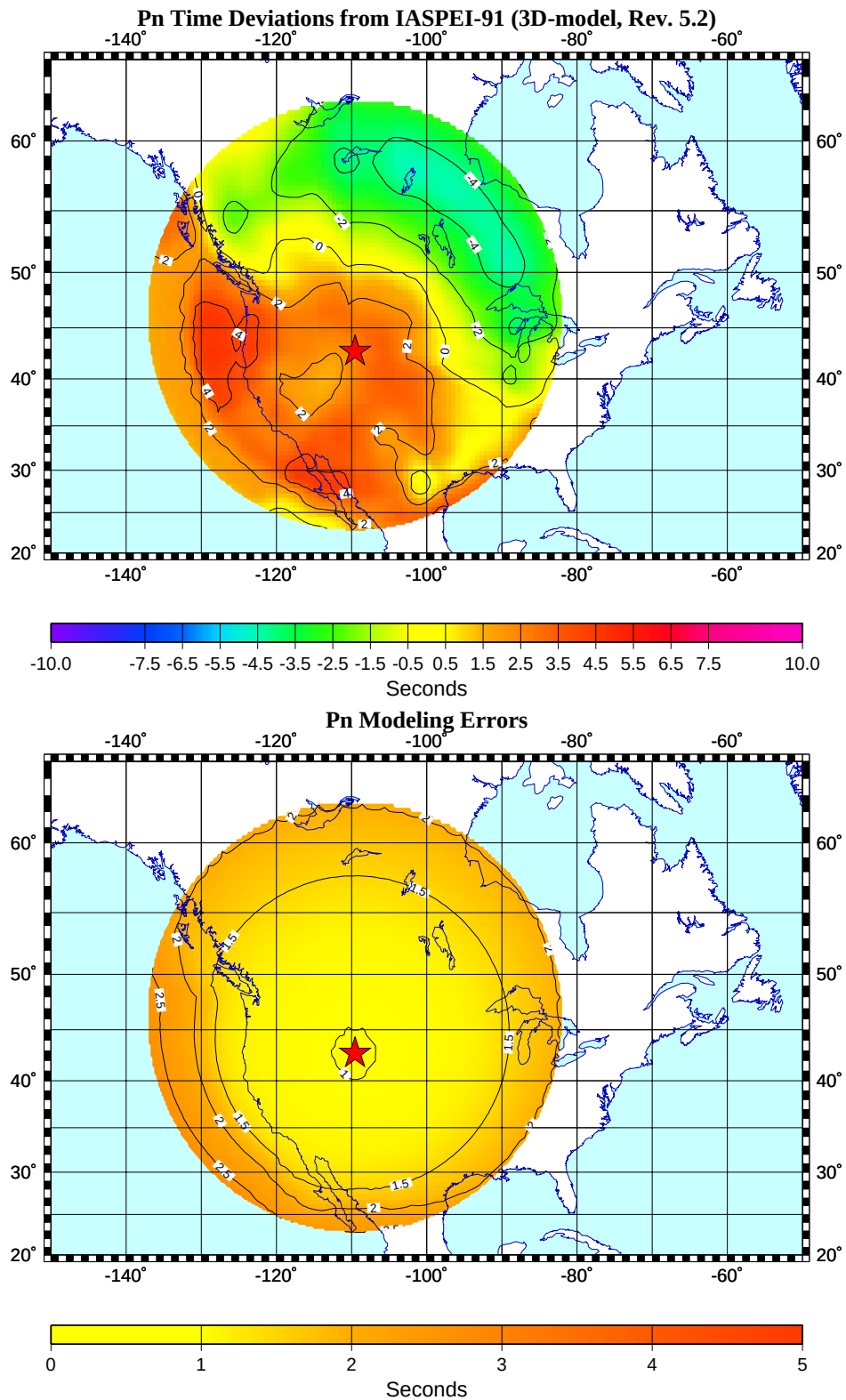
Figure 3. PDAR station, North America. Pn SSSCs and modeling errors.
