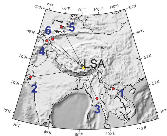
Figure 8. Love-wave dispersion curves for 6 paths from station LSA across southeast Asia.
