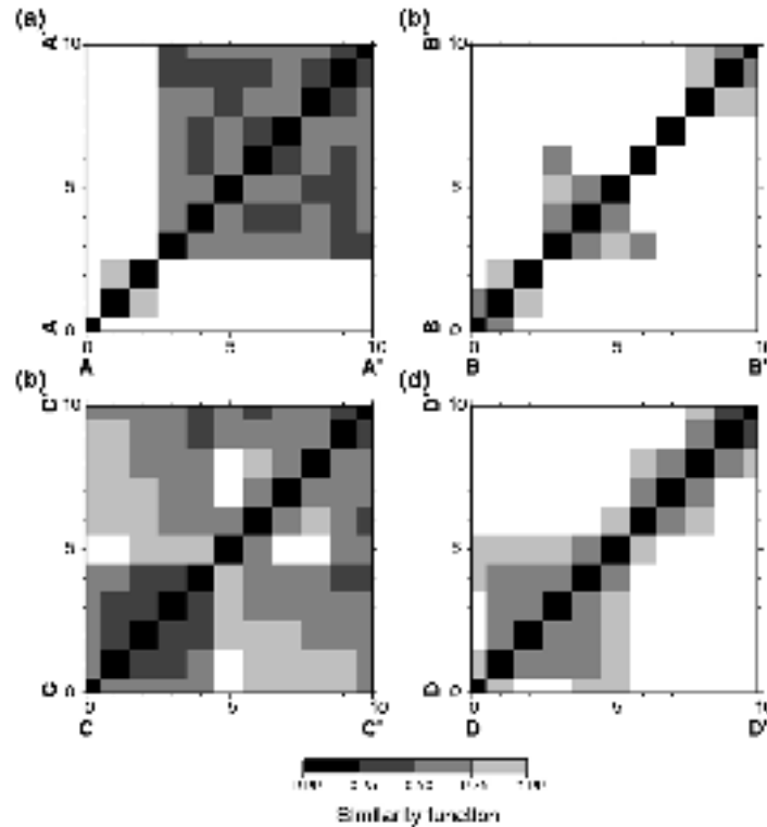
Figure 7. Similarity matrices calculated for the profiles shown in Figure 4. Similarity function is defined by equation 4. Dark shades denote high similarity between the 1-D models at the corresponding spatial locations.
